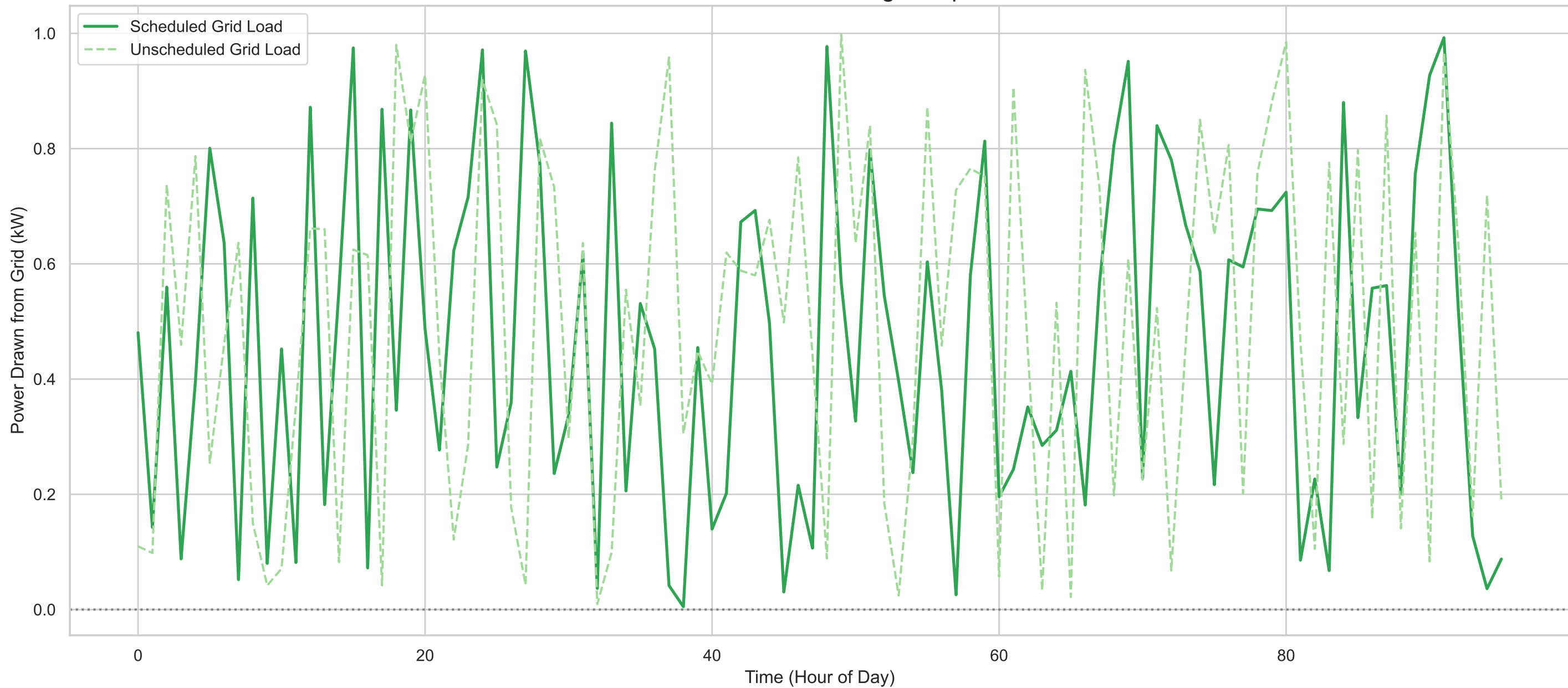
Case 1: Grid Peak Shaving Comparison
