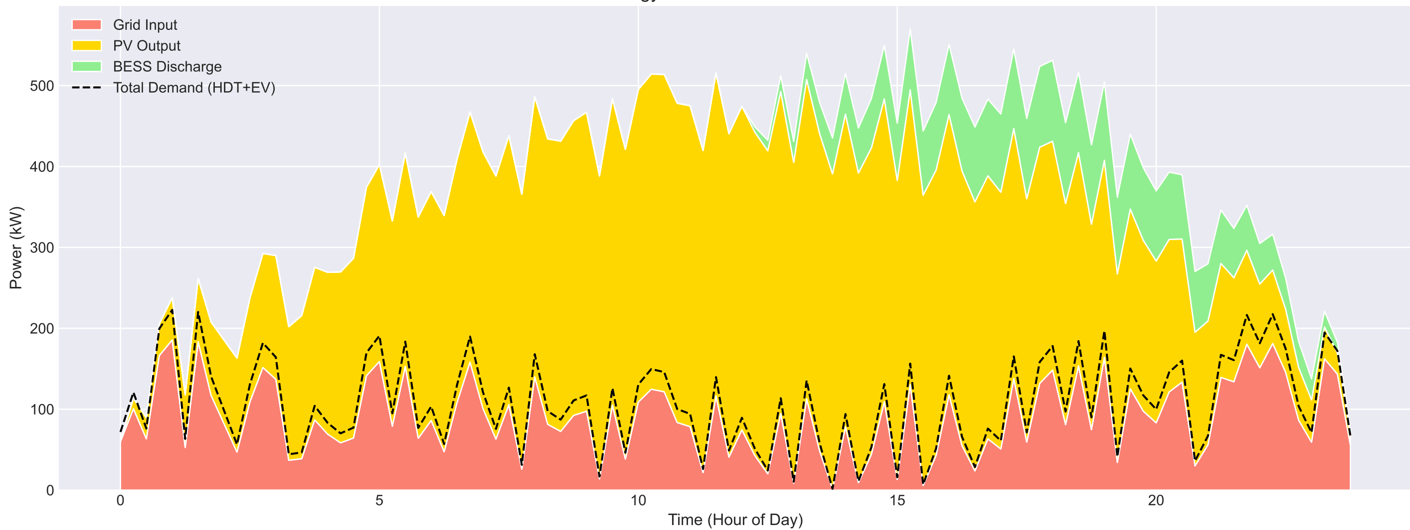
Energy Flow: Unscheduled Fleet
