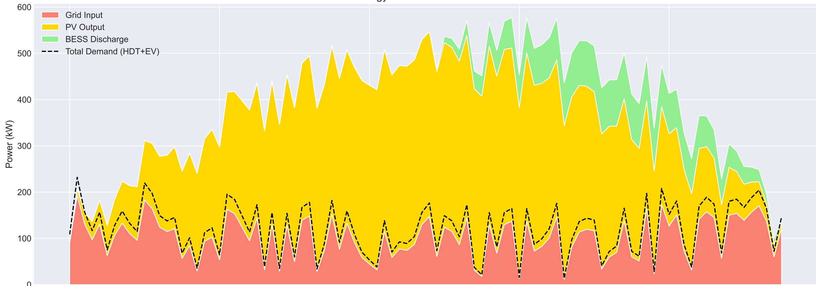
Energy Flow: Unscheduled Fleet
