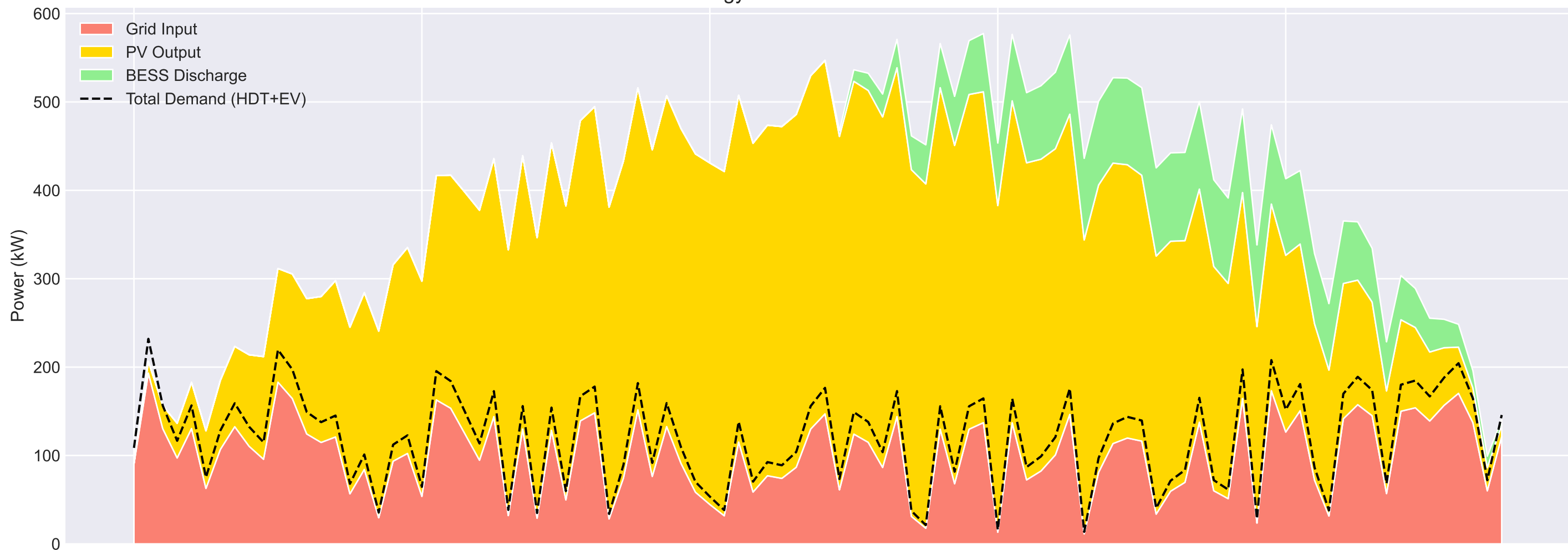
Energy Flow: Scheduled Fleet
