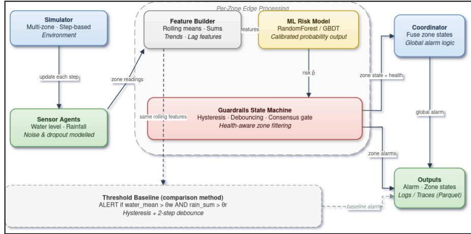
Fig 1. Architecture of the Multi-Agent System
