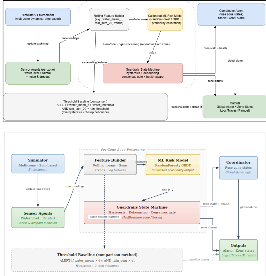
Fig 1. Architecture of the Multi-Agent System
