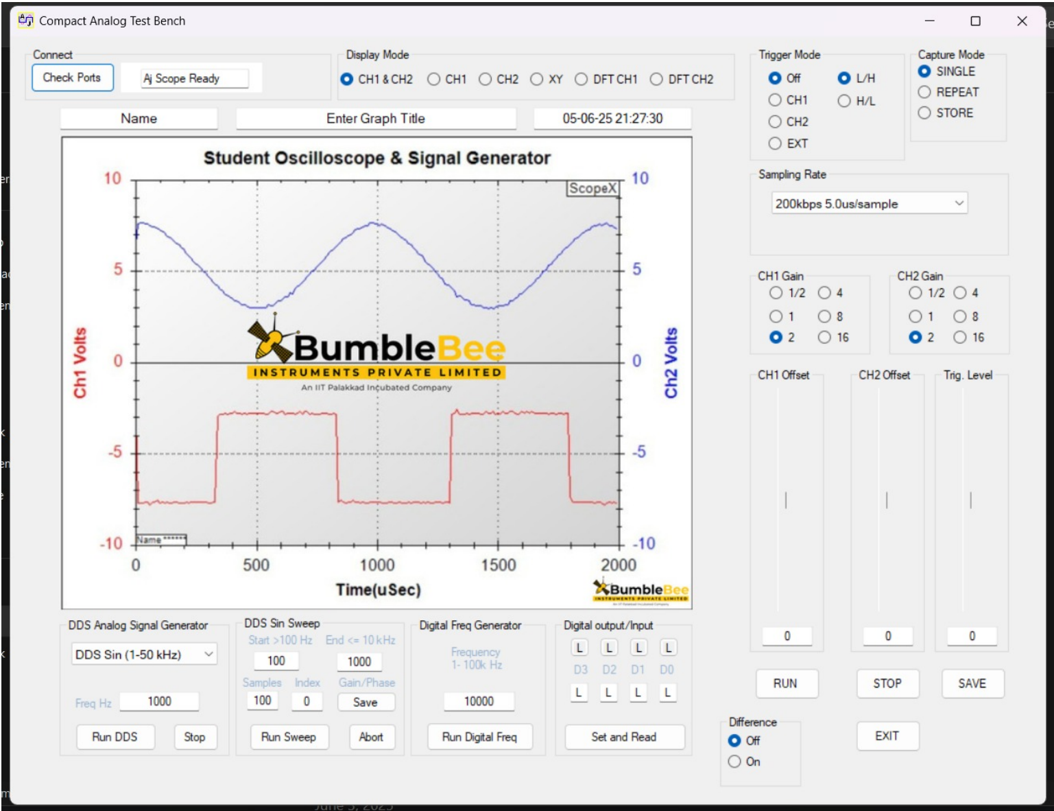
Figure 7: Launch the GUI and click 'Check Ports'.The device is now successfully connected.
