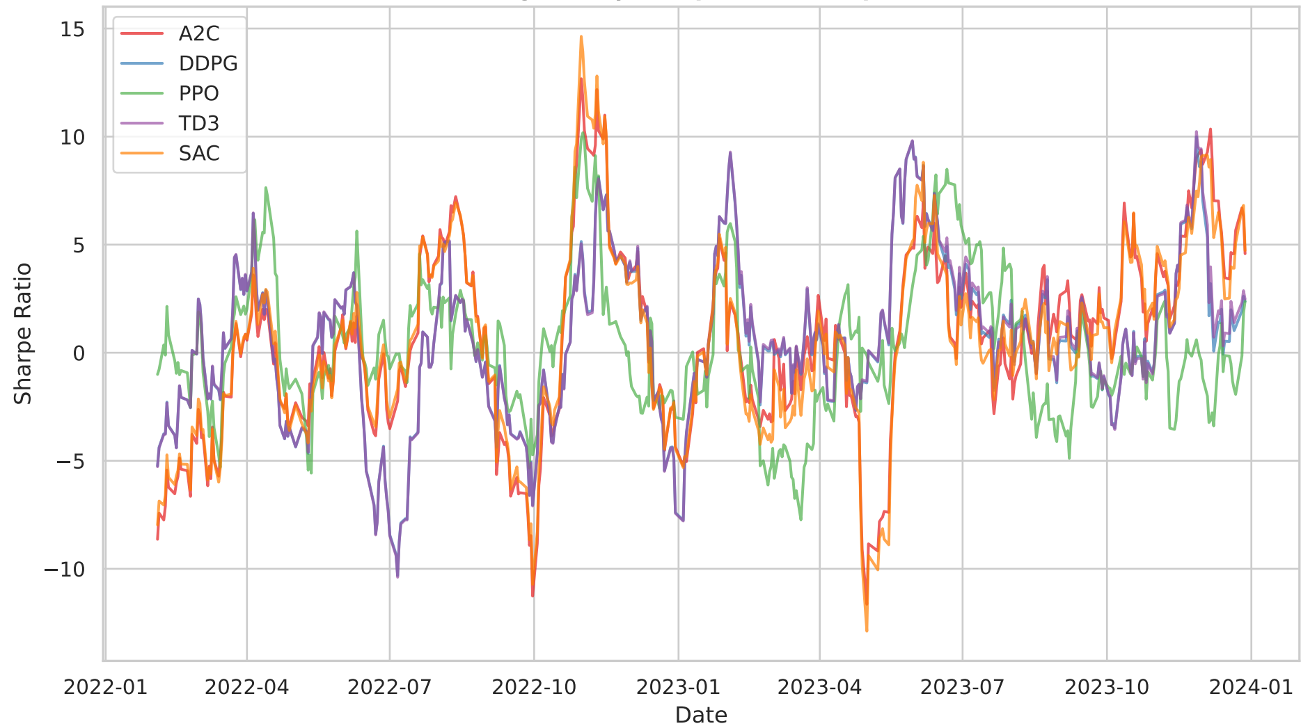
Rolling 20-Day Sharpe Ratio Comparison
