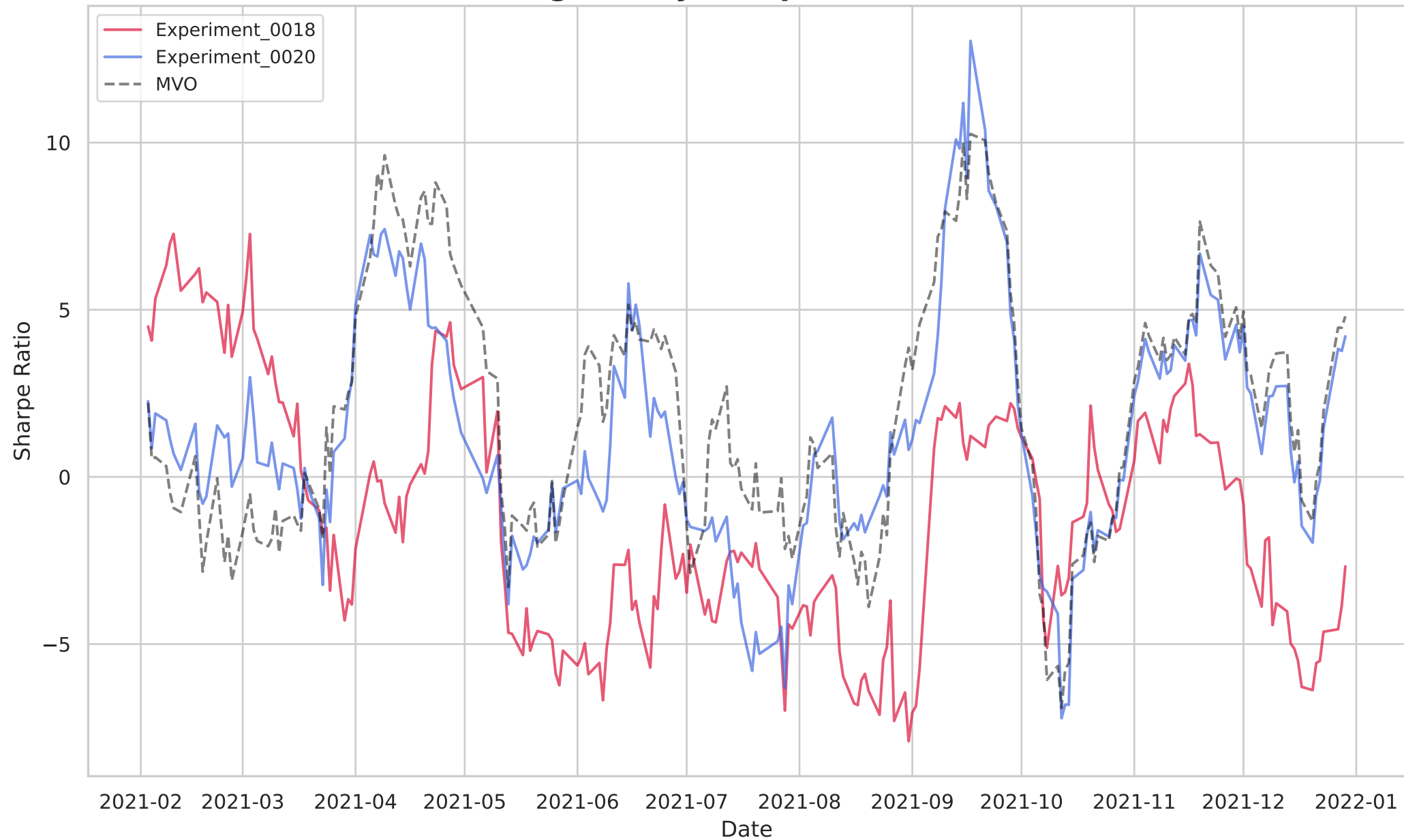
SAC - Rolling 20-Day Sharpe Ratio (Annualized)
