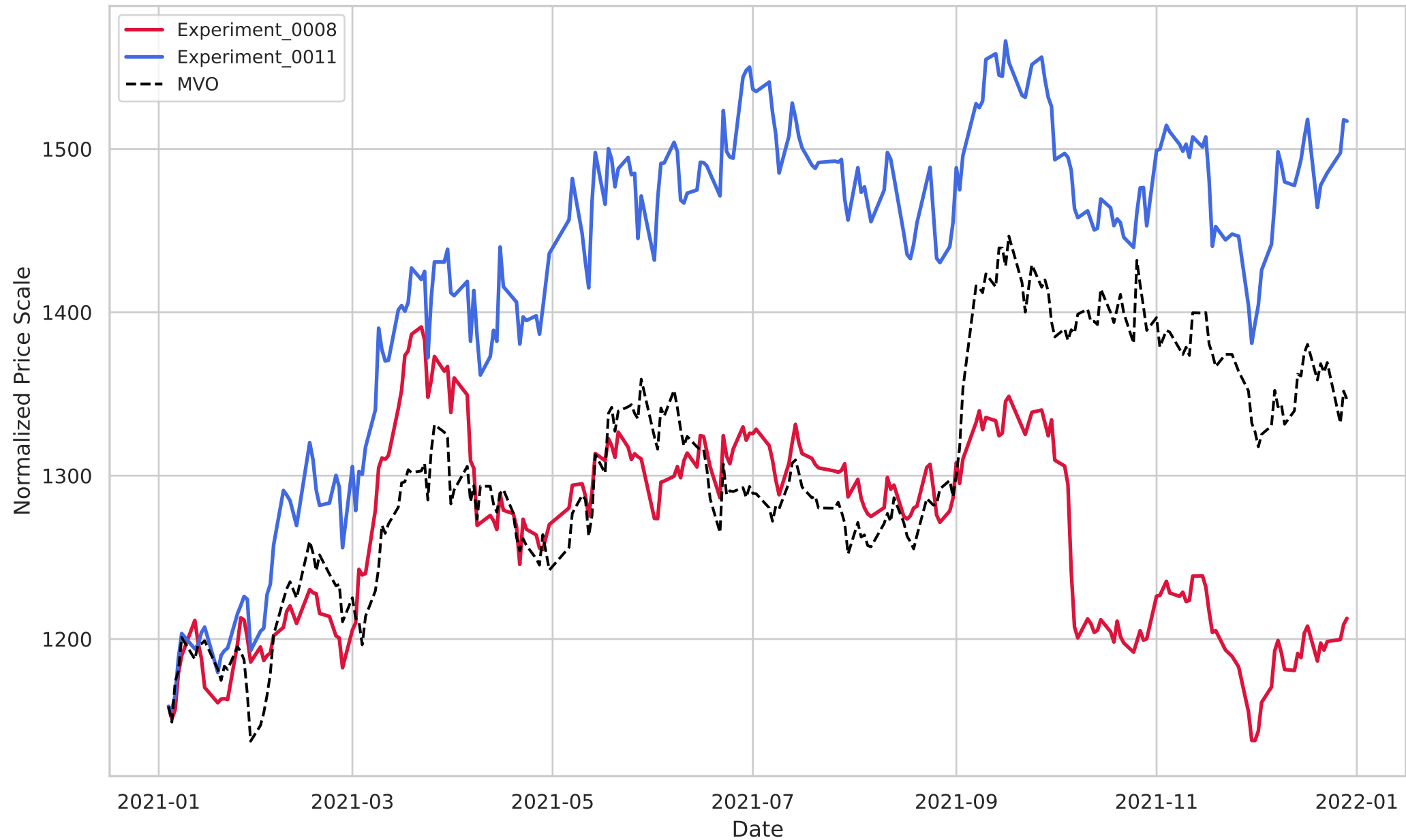
DDPG - Portfolio Value Over Time
