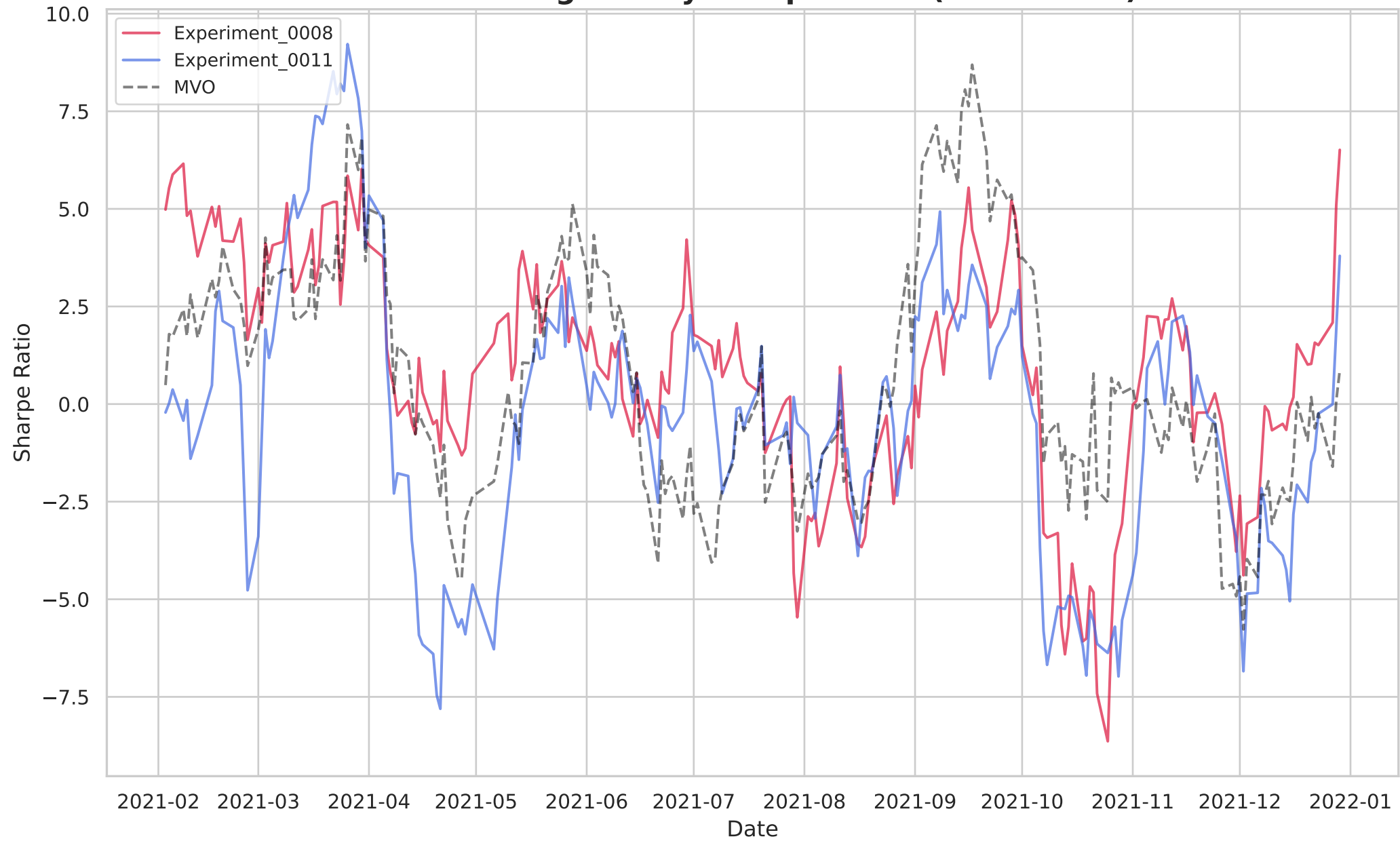
TD3 - Rolling 20-Day Sharpe Ratio (Annualized)
