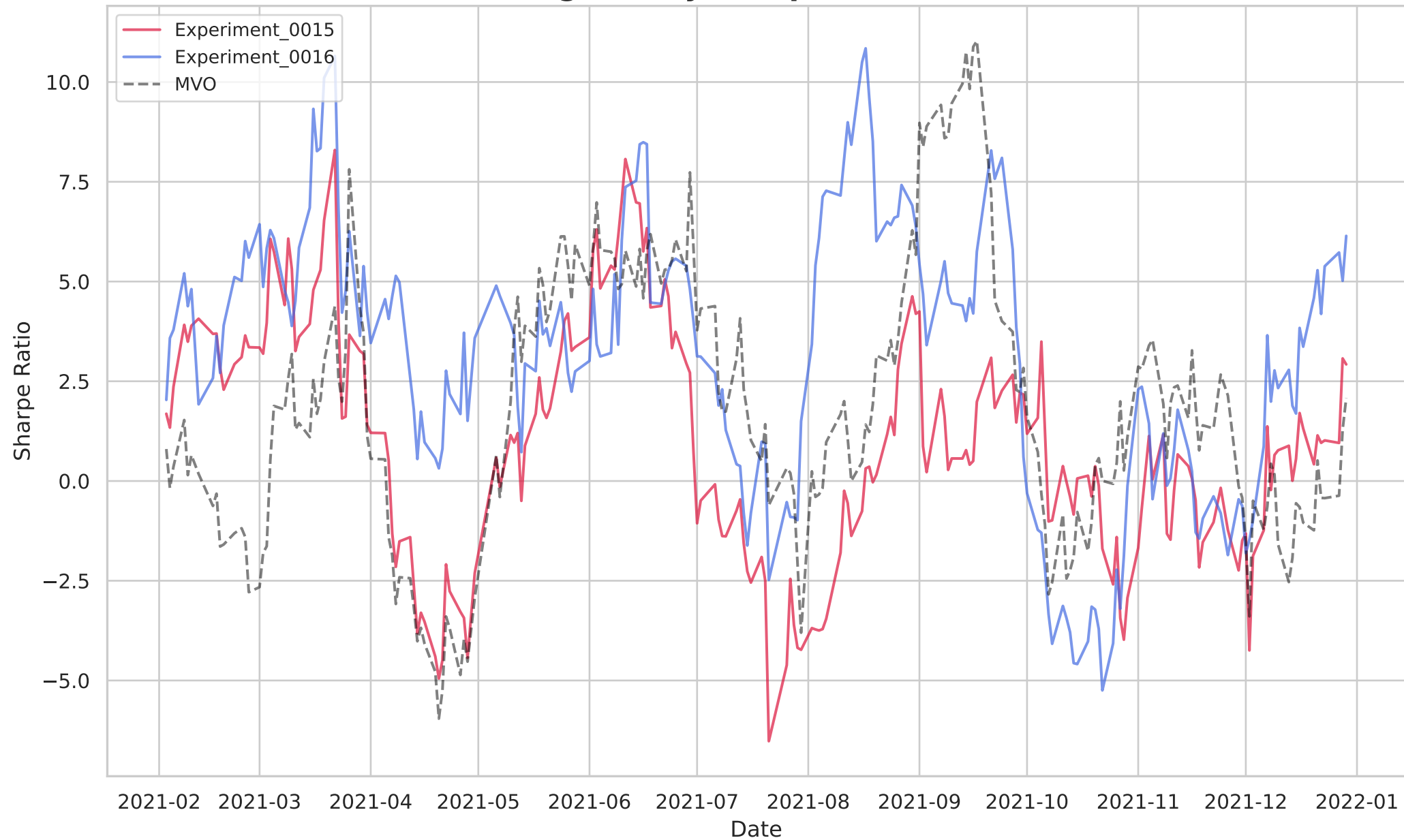
A2C - Rolling 20-Day Sharpe Ratio (Annualized)
