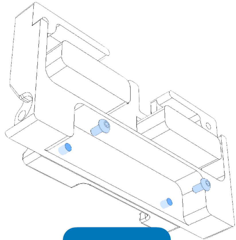
2* M3*6mm BHCS
