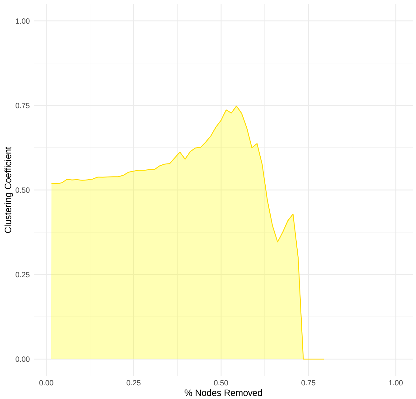
Global Clustering Coefficient During Node Removal – Degree
