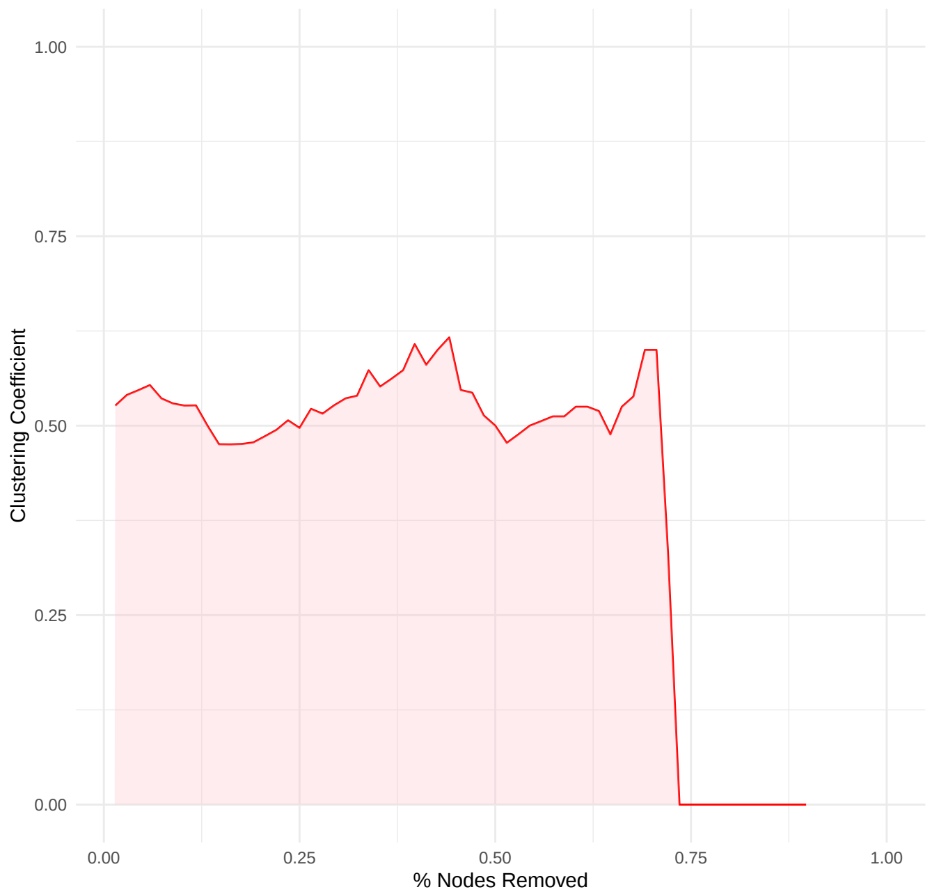
Global Clustering Coefficient During Node Removal – Closeness
