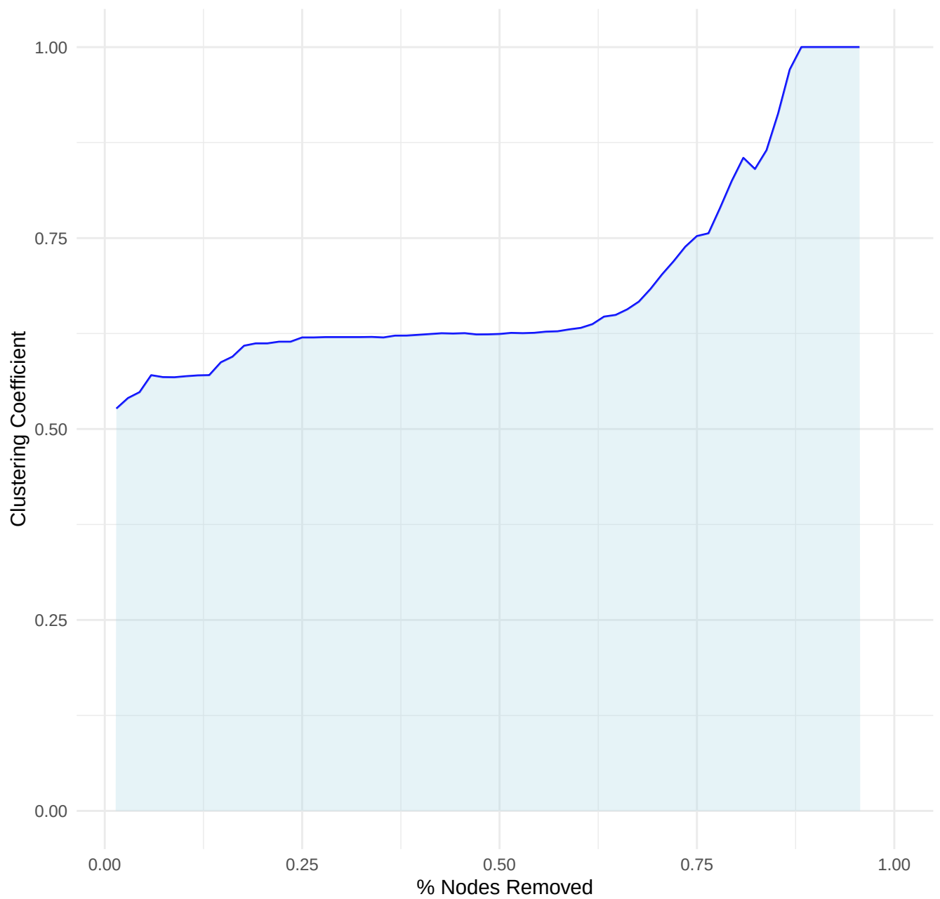
Global Clustering Coefficient During Node Removal – Eigenvector
