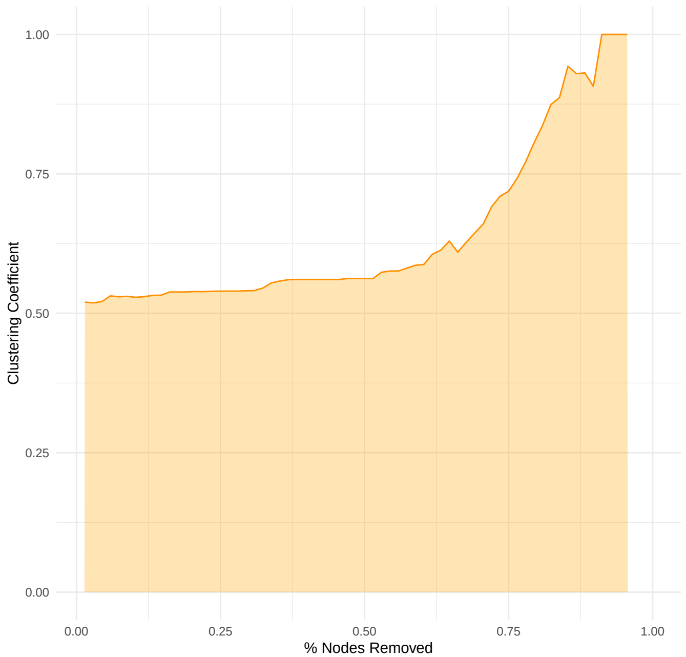
Global Clustering Coefficient During Node Removal – Modularity
