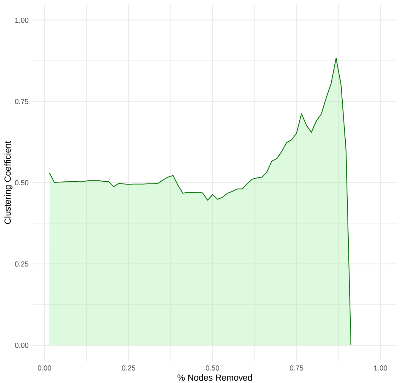
Global Clustering Coefficient During Node Removal – Betweenness
