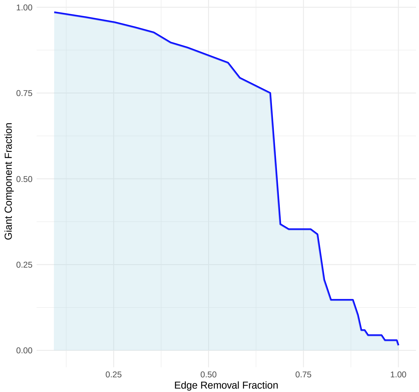
Robustness Analysis (AUC = 0.5828)
