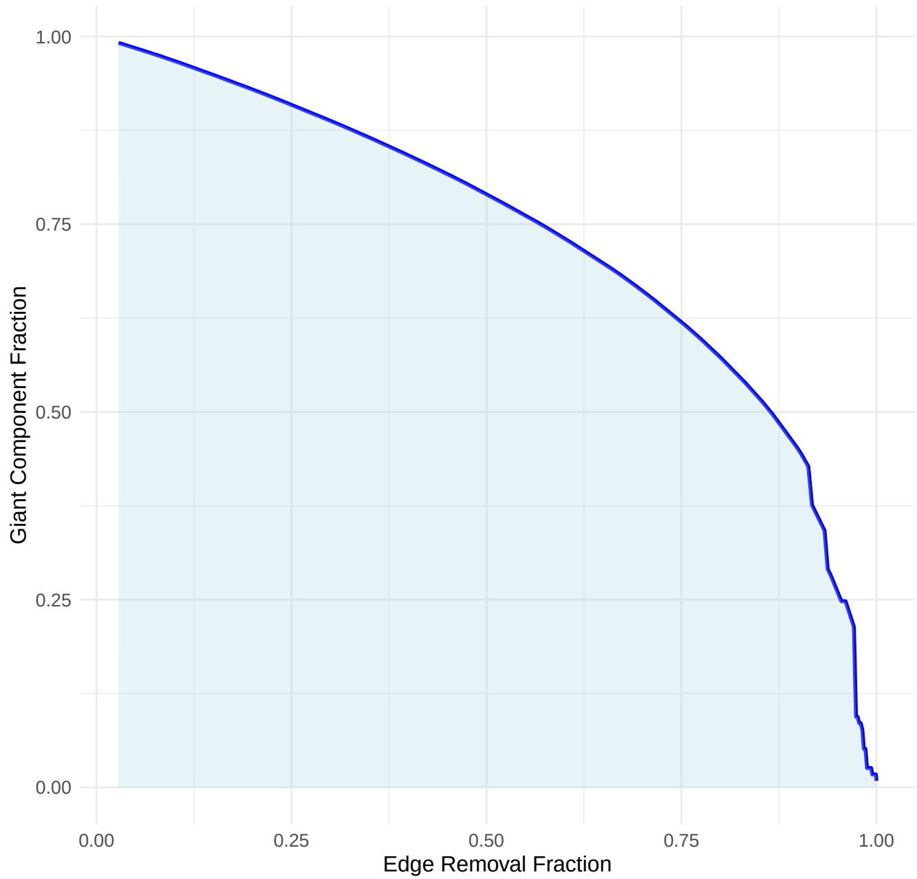
Robustness Analysis (AUC = 0.708)
