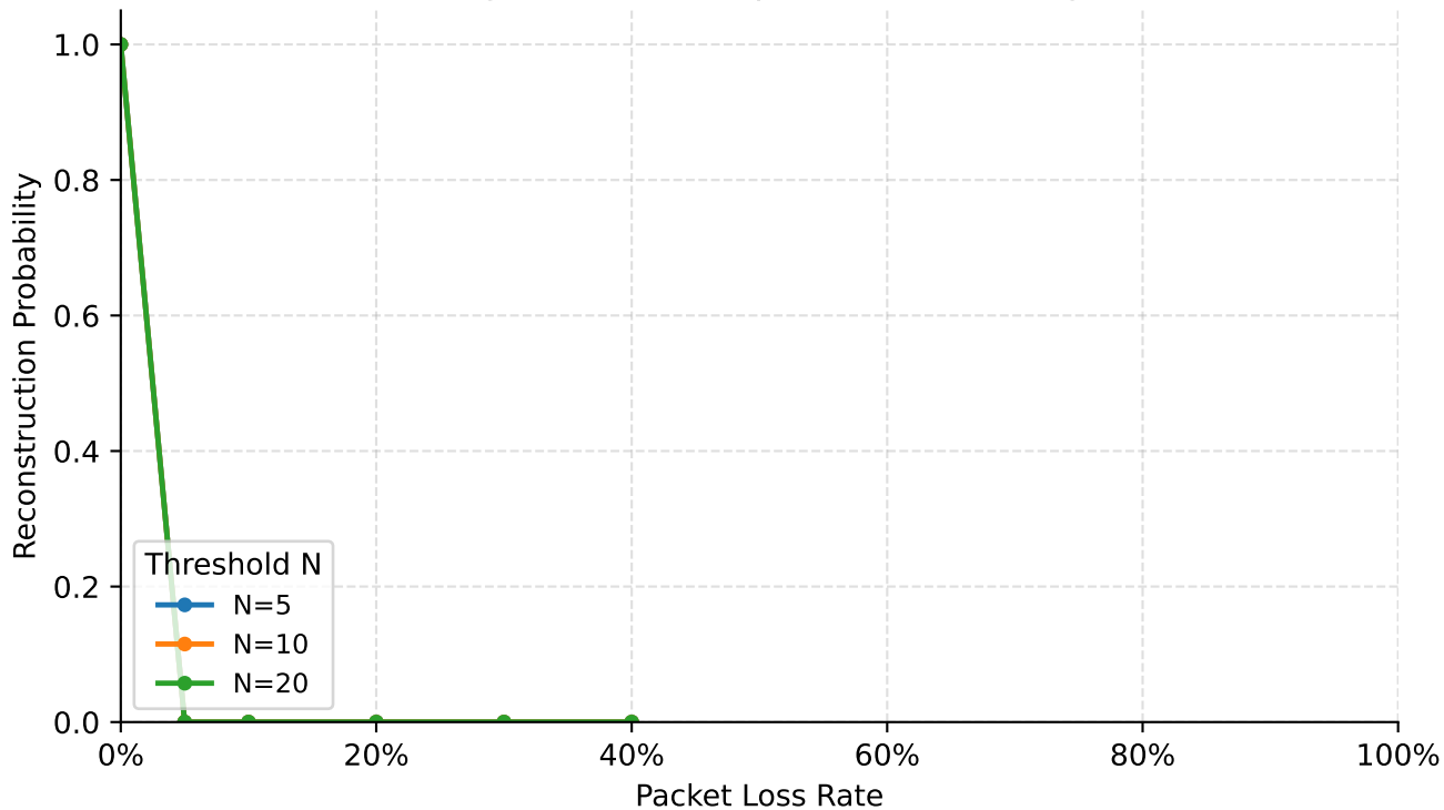
Reconstruction Probability vs Packet Loss (Aegis-Grid v2 Adaptive Thresholding)
