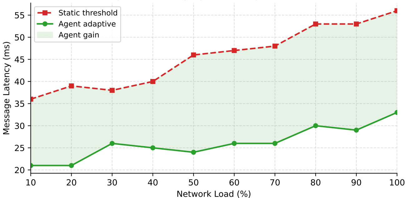
Static vs Agent-Adaptive Latency Under Load (Agent advantage grows at high load — v3)
