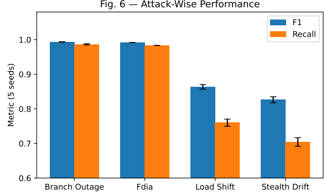
Fig. 6. Five-seed mean F1 and recall across the validated attack scenarios.
