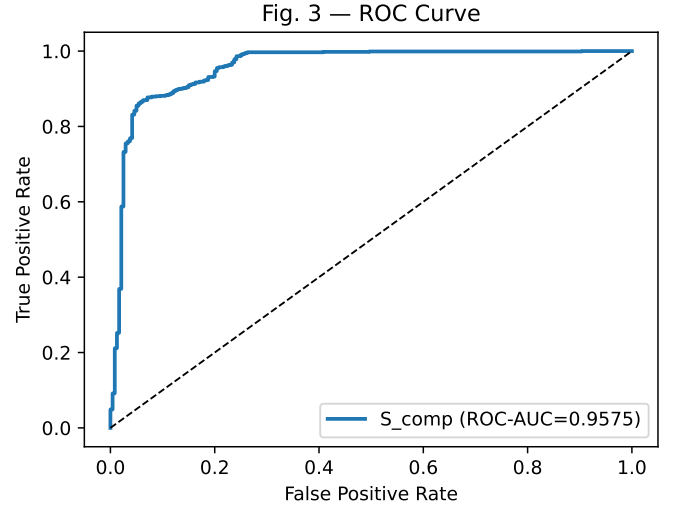
Fig. 3. ROC curve for the continuous composite threat score.
