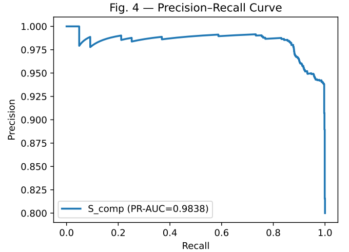
Fig. 4. Precision-recall curve for the continuous composite threat score.
