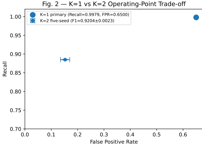
Fig. 2. K = 1 versus K = 2 operating-point trade-off using the validated detector outputs and five-seed aggregate summary.
