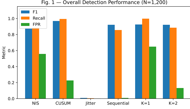
Fig. 1. Overall detection-performance comparison for the primary validation set.
