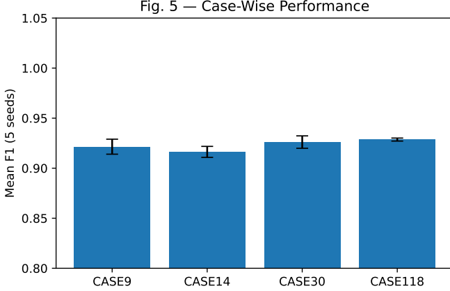
Fig. 5. Five-seed mean F1 performance across the four IEEE benchmark topologies.
