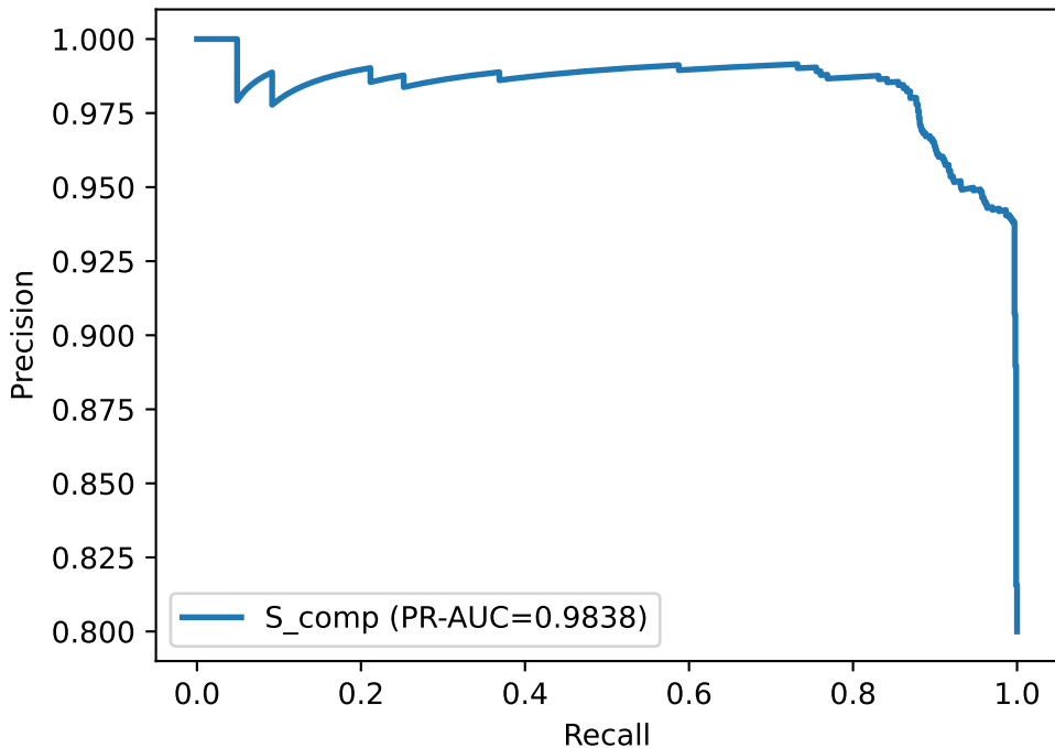
Fig. 4 — Precision-Recall Curve
