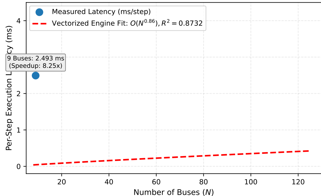
Fig. 11 — Computational Latency & Empirical Scaling
