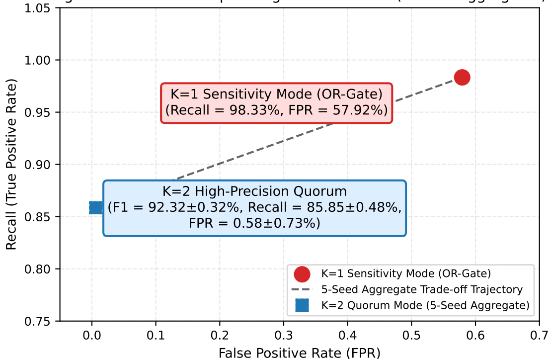
Fig. 2 — K=1 vs K=2 Operating-Point Trade-off (5-Seed Aggregates)
