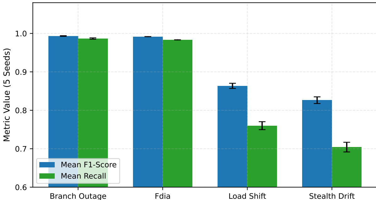
Fig. 6 — Attack-Wise Performance Across Scenarios
