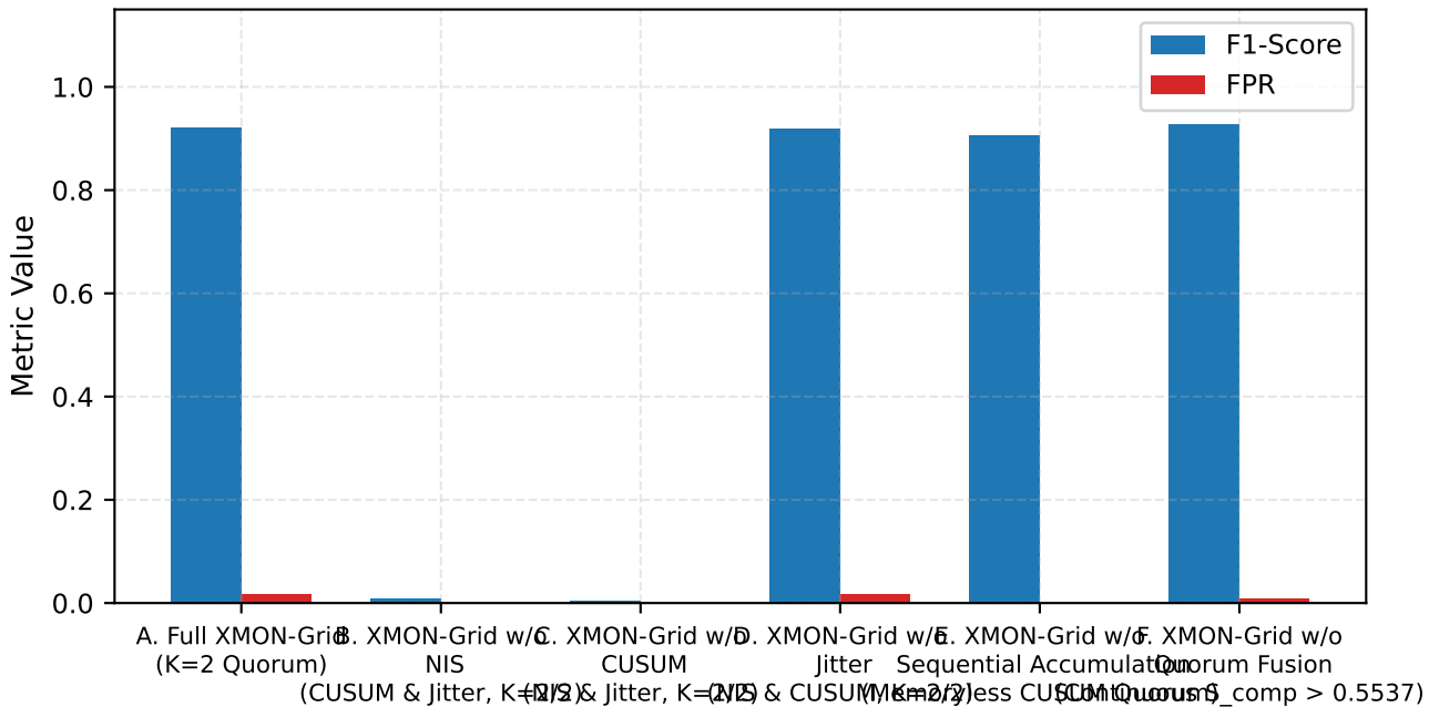
Fig. 7 — Component Ablation Study (Ablations A-F)
