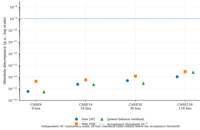
Fig. 8. Independent AC power-flow consistency check for the canonical IEEE benchmark systems. The plotted quantities are the maximum absolute active-power residual, maximum absolute reactive-power residual, and absolute network power-balance residual reconstructed from the canonical admittance model; values are shown on a logarithmic scale in per-unit.
