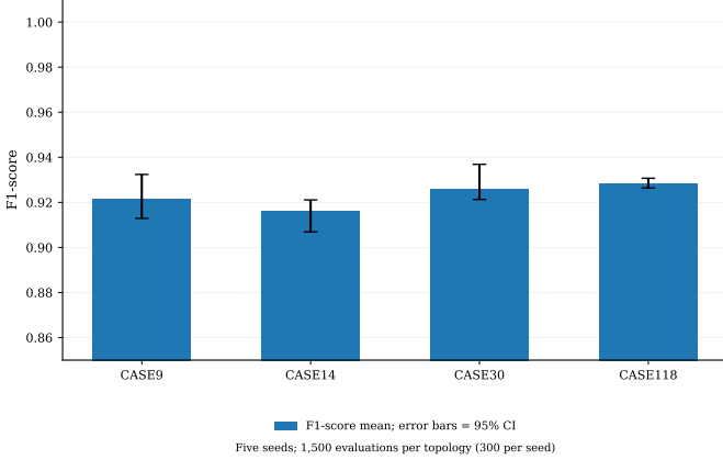
Fig. 5. Topology-wise K = 2 F1-score across IEEE 9-, 14-, 30-, and 118-bus benchmarks. Bars are five-seed means; error bars are the authoritative 95% confidence intervals. Each topology contributes 1,500 evaluations (300 per seed).
