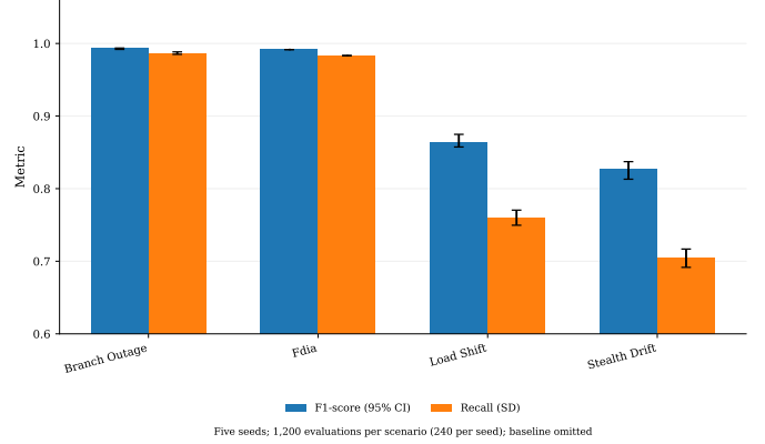
Fig. 6. Attack-wise K = 2 performance for branch outage, FDIA, load shift, and stealth drift. F1 bars use authoritative 95% confidence intervals; recall bars use five-seed standard deviations. Each scenario contributes 1,200 evaluations (240 per seed); the benign baseline is excluded from the attack comparison.
