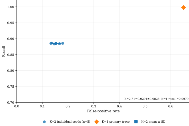
Fig. 2. K = 1 versus K = 2 operating-point trade-off. The diamond is the primary-trace K = 1 OR rule; individual circles are the five independent K = 2 seeds; the larger point and error bars show the five-seed mean \pm sample standard deviation. K = 2 is the strict majority of the three binary detector streams.
