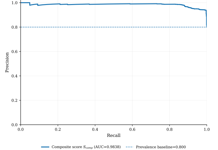
Fig. 4. Precision-recall curve for the continuous composite threat score S_{\text{comp}} , evaluated over all 6,000 authoritative test evaluations. The legend reports PR-AUC and the dashed horizontal line gives the positive-class prevalence baseline.
