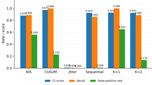
Fig. 1 — Overall Detection Performance (N=1,200; 960 positive, 240 negative)
