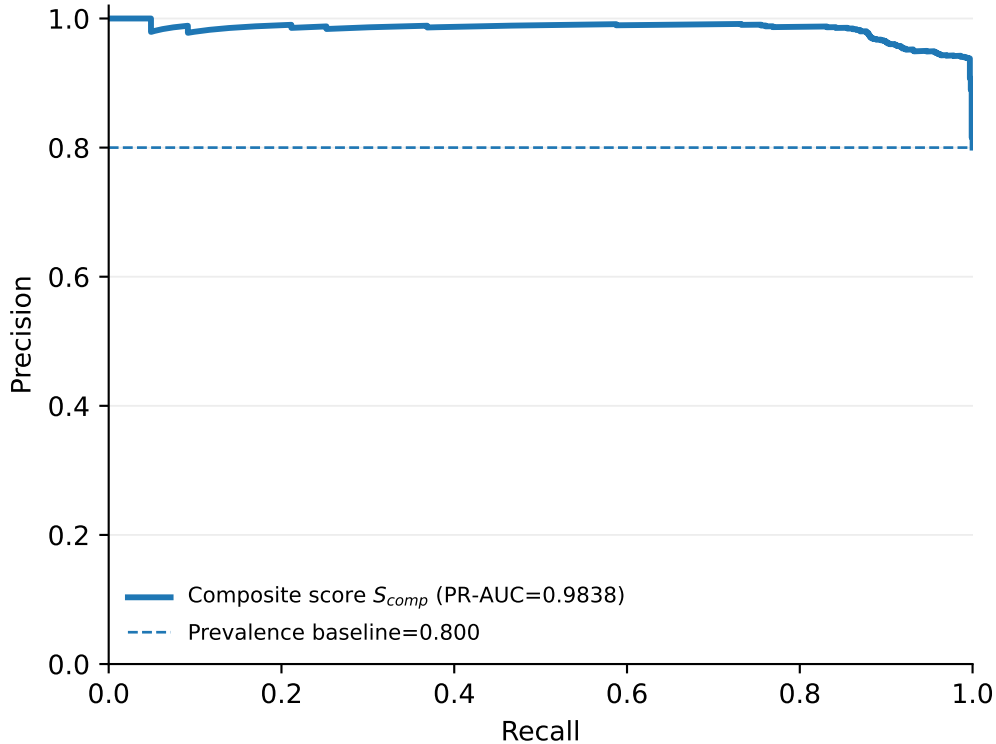
Fig. 4 — Precision-Recall Curve (N=1,200)
