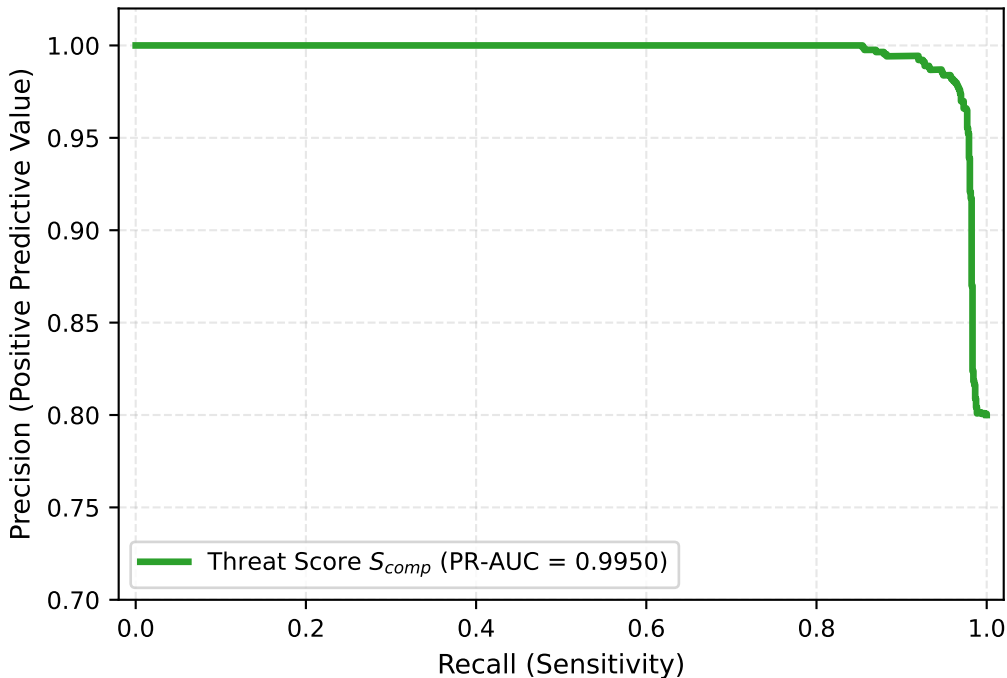
Fig. 4 — Precision-Recall (PR) Curve
