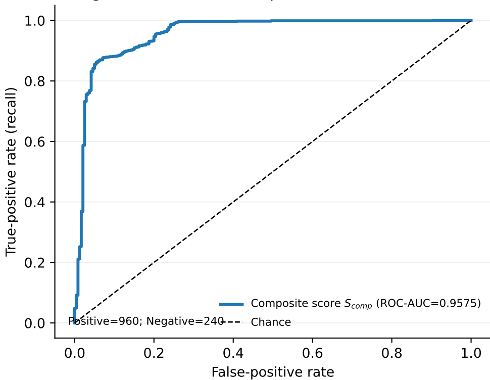
Fig. 3 — Threshold-Independent ROC (N=1,200)
