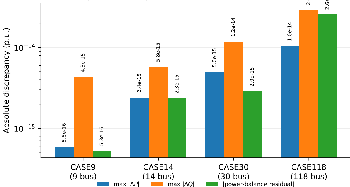
Fig. 12 — Independent AC Power-Flow Consistency
