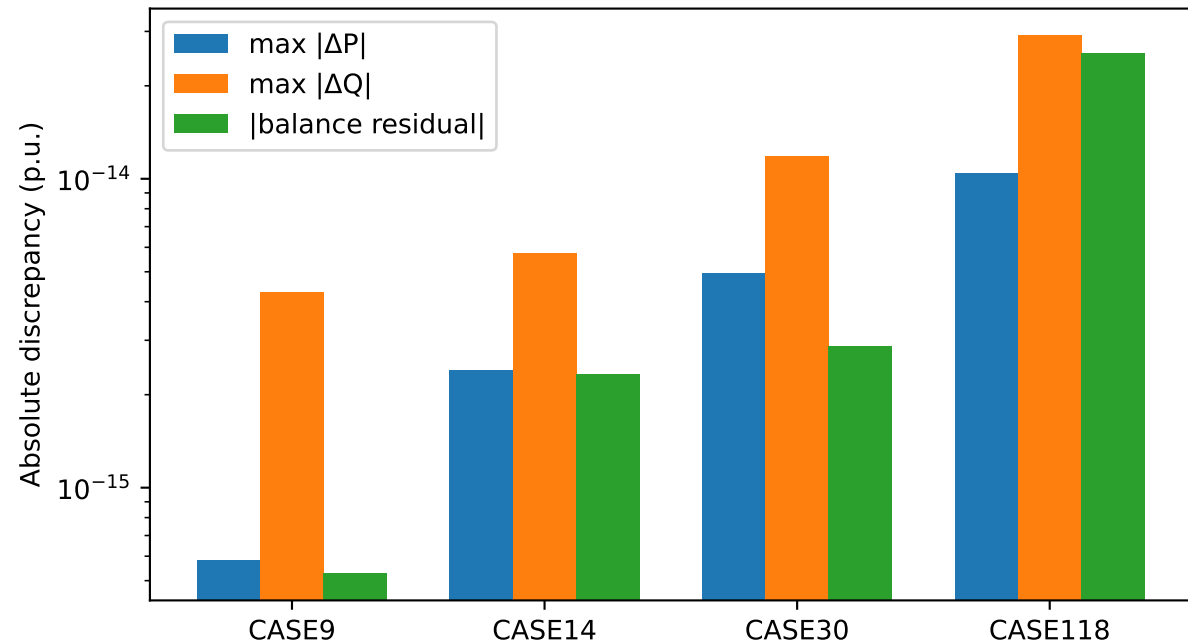
Fig. 12 — AC Power-Flow Numerical Consistency
