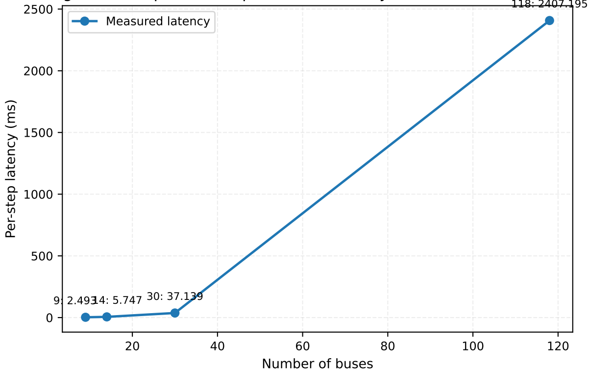
Fig. 11 — Empirical Computational Latency Across Benchmark Sizes
