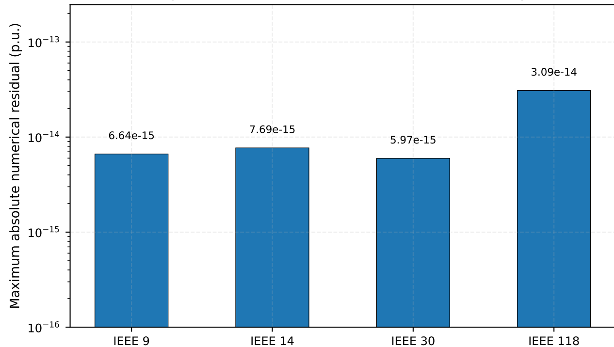
Fig. 12 — AC Power-Flow Numerical Consistency
