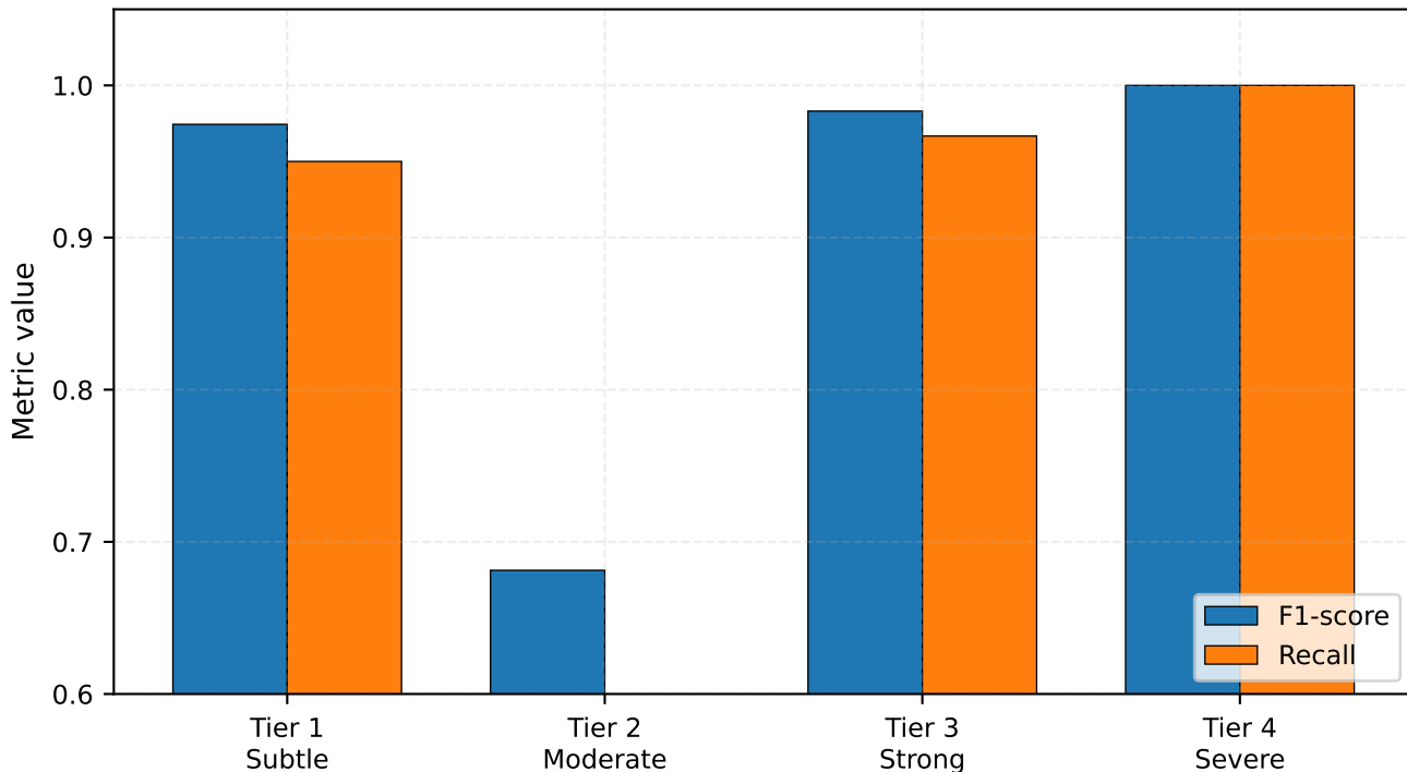
Fig. 10 — Attack-Severity Spectrum Robustness
