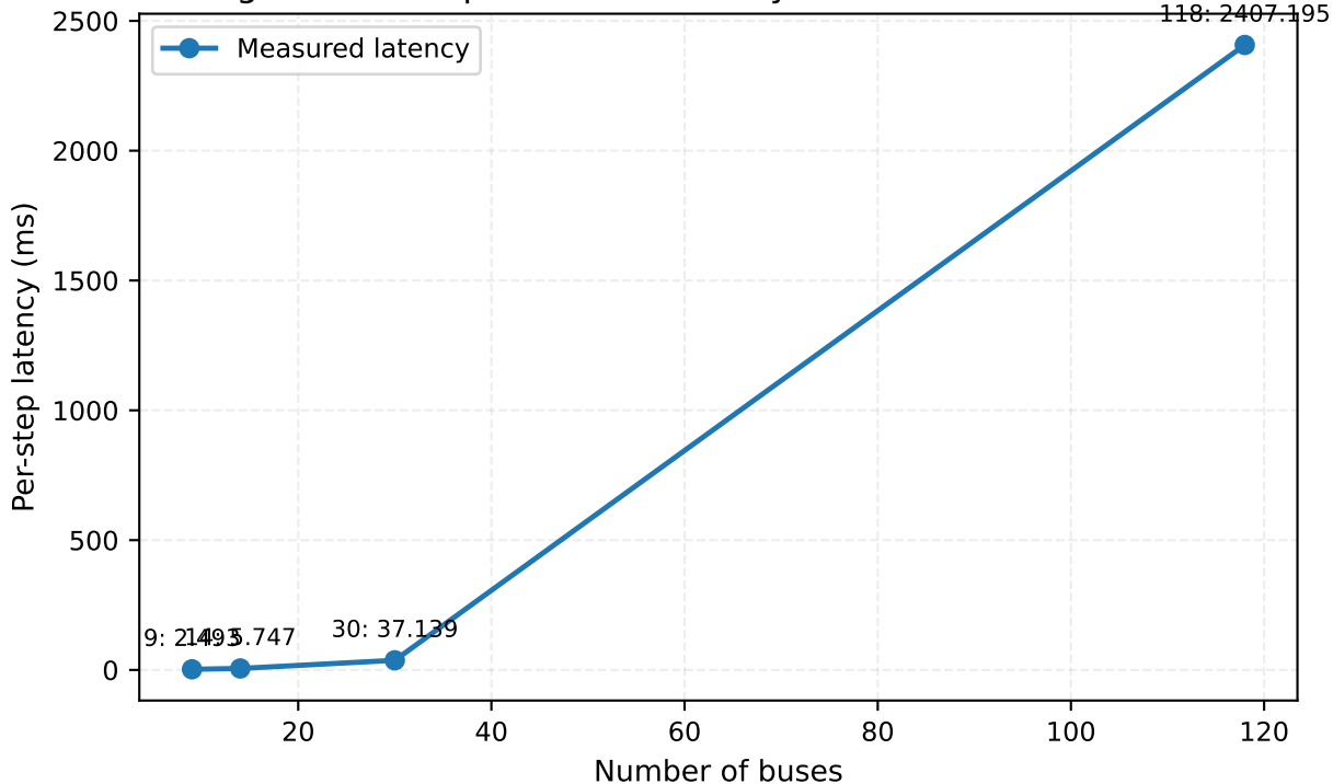
Fig. 11 — Computational Latency Across Benchmark Sizes
