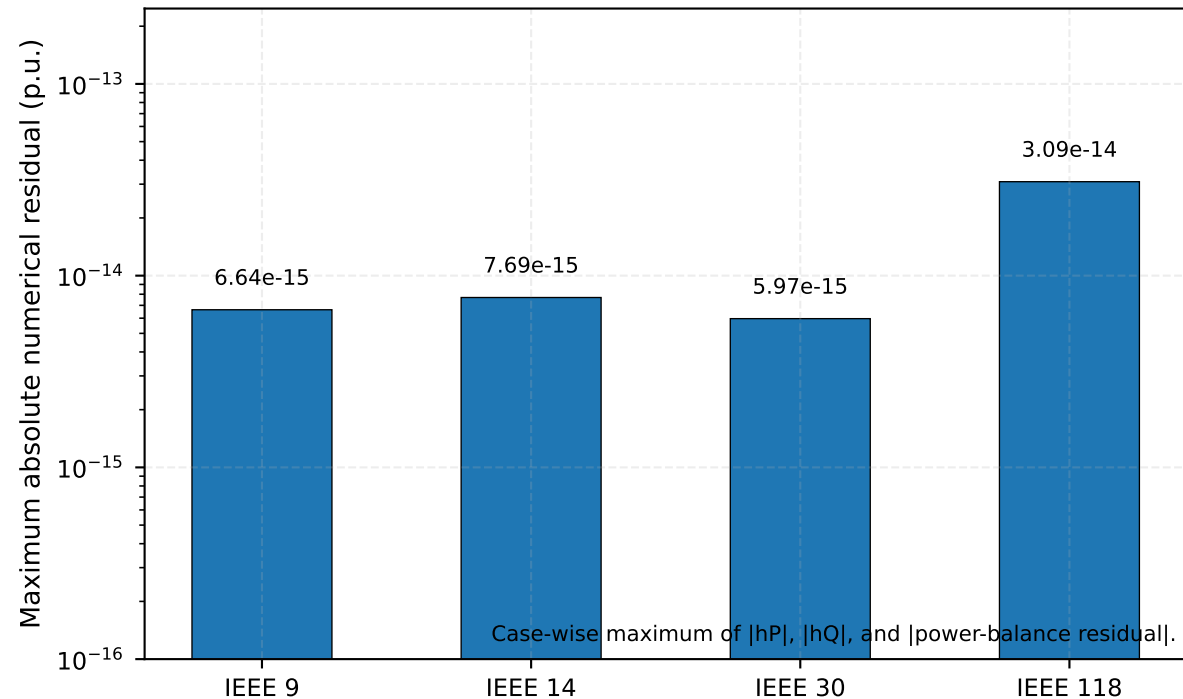
Fig. 12 — AC Power-Flow Numerical Consistency
