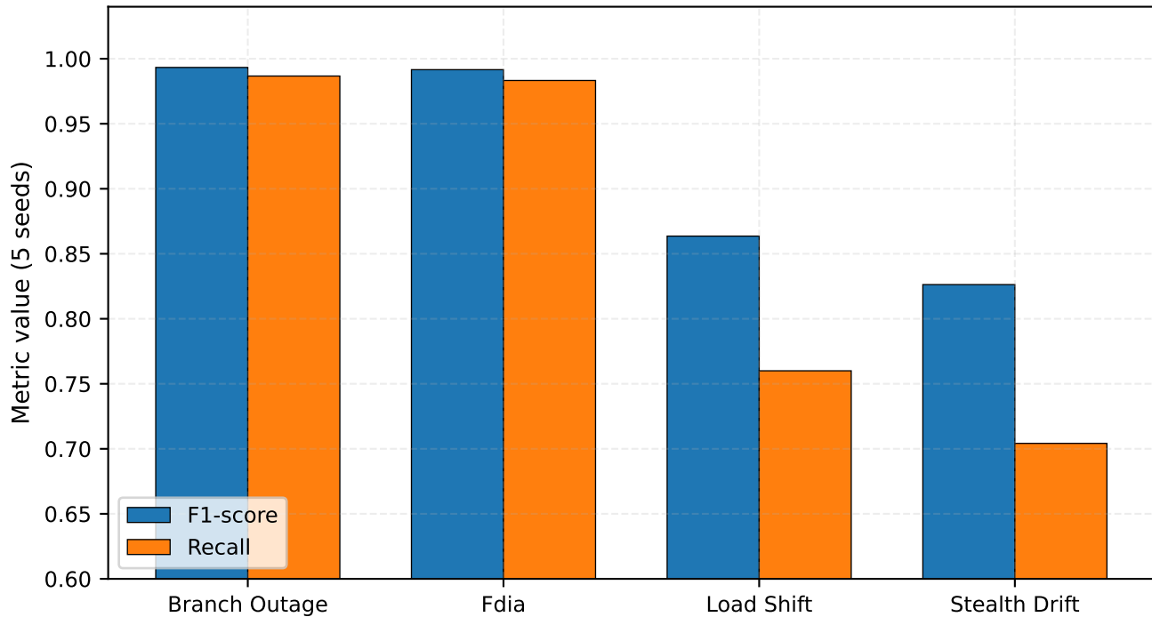
Fig. 6 — Attack-Wise Performance
