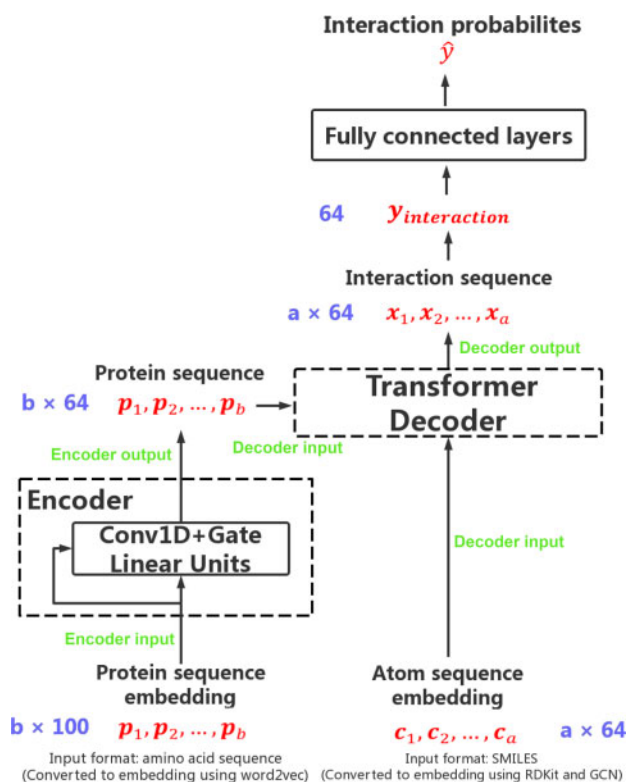
Fig. 2. Computational graph of TransformerCPI
