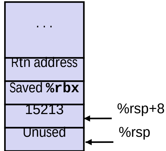
Pre-return Stack Structure
