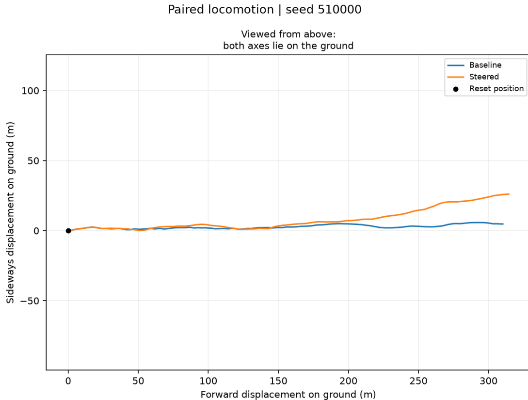
Figure 2. Top-down displacement for the first predetermined validation seed, 510000, comparing zero steering with lateral alpha -0.1. Both axes lie on the ground and use equal physical scale. Positions are reconstructed from saved velocities and timestep relative to reset. This is one existing validation example, not a fresh application test.
