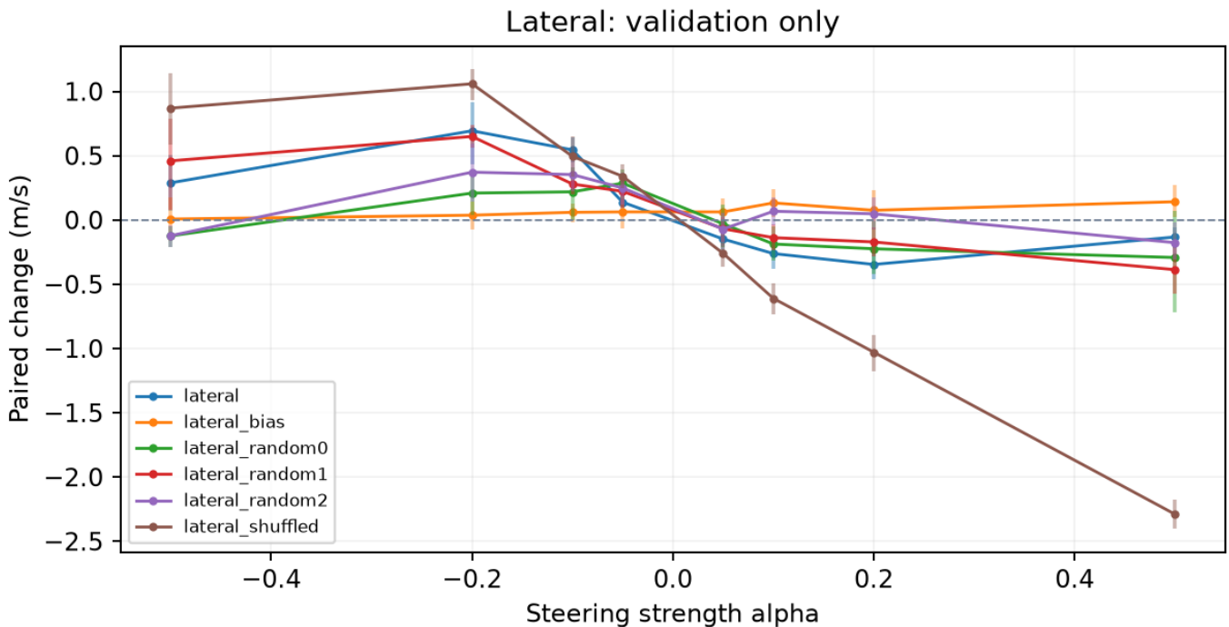
Figure 1. Ant lateral validation strength response. Every primary and random/shuffled activation setting is shown; error bars are paired-episode percentile intervals. The separate action-bias comparator was calibrated after a primary qualified.
