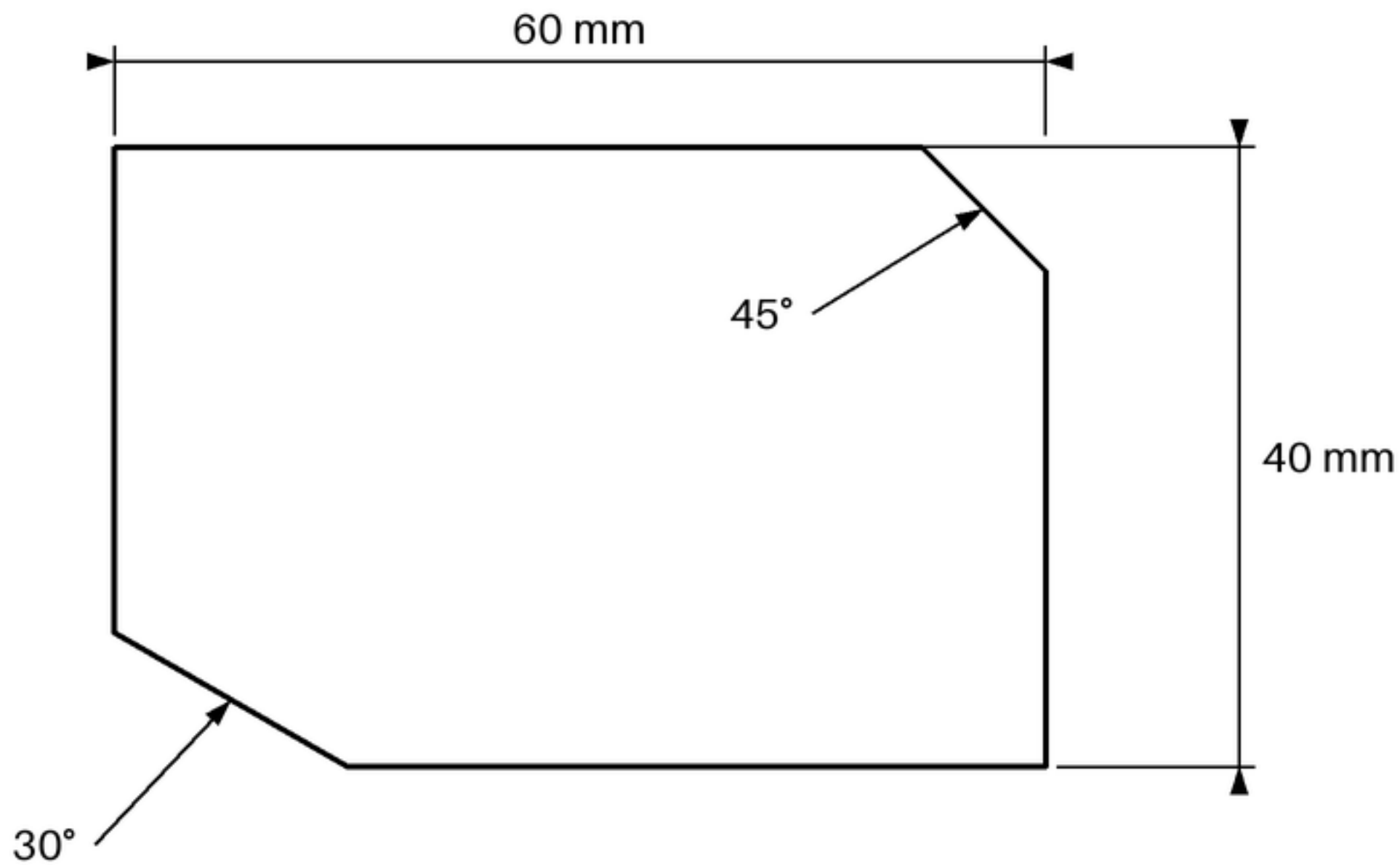
CHAMFER AND ANGLE CUT
