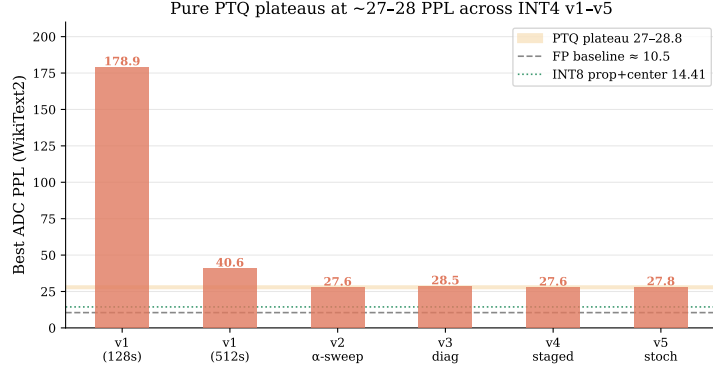
Figure 3: Pure PTQ plateau. After all transform-based PTQ improvements (sample count, \alpha -mixing, diagonals, staged training), INT4 ADC perplexity saturates around 27.5–28.5, independent of calibration strategy. The remaining gap to the FP and INT8 baselines motivates the post-ADC residual correction stage.
