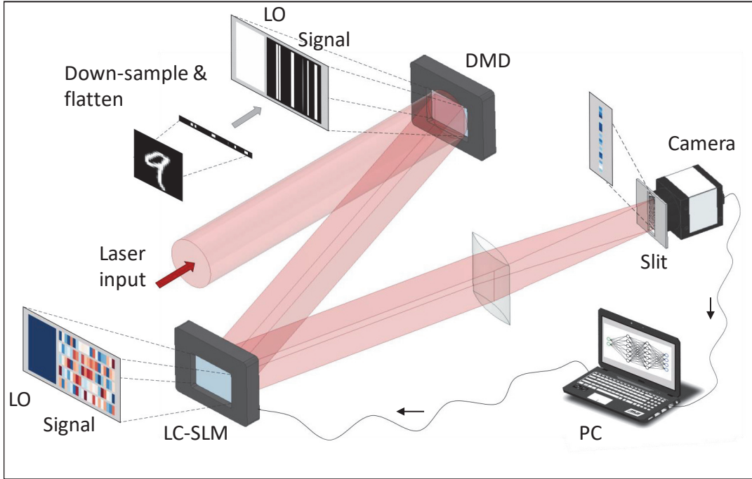
Figure 1: Physical example of an analog matrix–vector multiplication feeding an ADC. The figure, reproduced from Spall, Guo, and Lvovsky [27], shows an optical neural-network front-end: weights and activations are encoded into light fields, the inner product is computed by optical interference, and the analog accumulator output is read by a photodetector before being sampled by an ADC. The same analog-input–ADC-output structure underlies electronic in-memory computing crossbars; the mathematical model in Eqs. (6)–(7) abstracts both.
