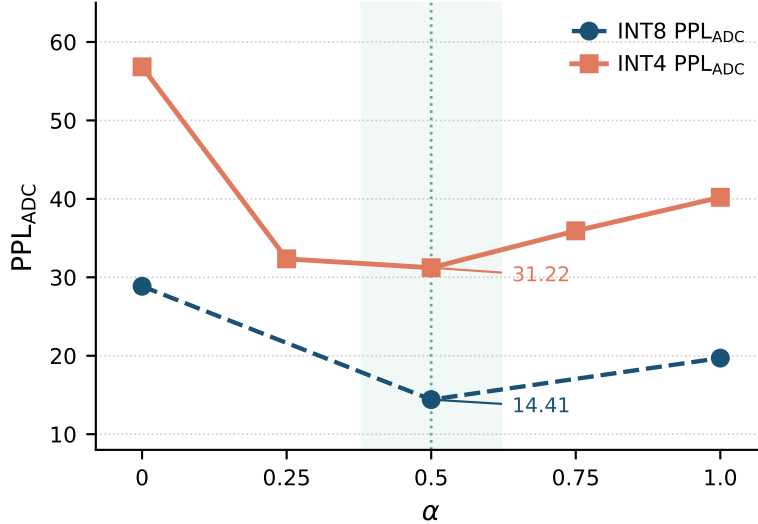
Figure 6: \alpha -mixing sweep at 1024 calibration samples. ADC PPL is minimized at \alpha = 0.5 ; smaller values under-weight the ADC regime, larger values amplify gradient noise from the floor operator and degrade no-ADC PPL.
