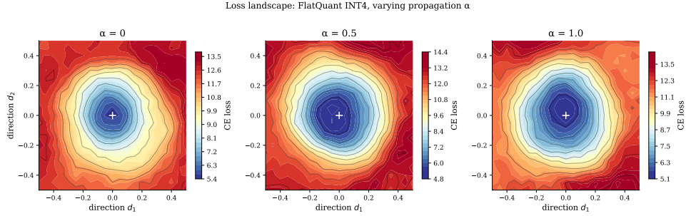
Figure 7: Loss-landscape visualisation around the converged transforms for \alpha \in \{0, 0.5, 1\} via filter-normalized random perturbations. The \alpha = 0.5 minimum is the widest and flattest, indicating that mixed FP/ADC calibration finds smoother solutions than either extreme.
