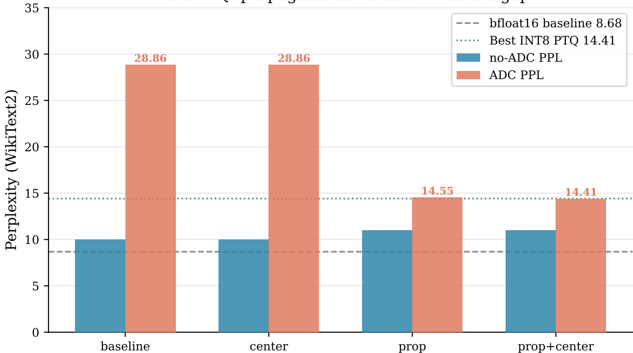
INT8 PTQ: propagated calibration fixes the gap
