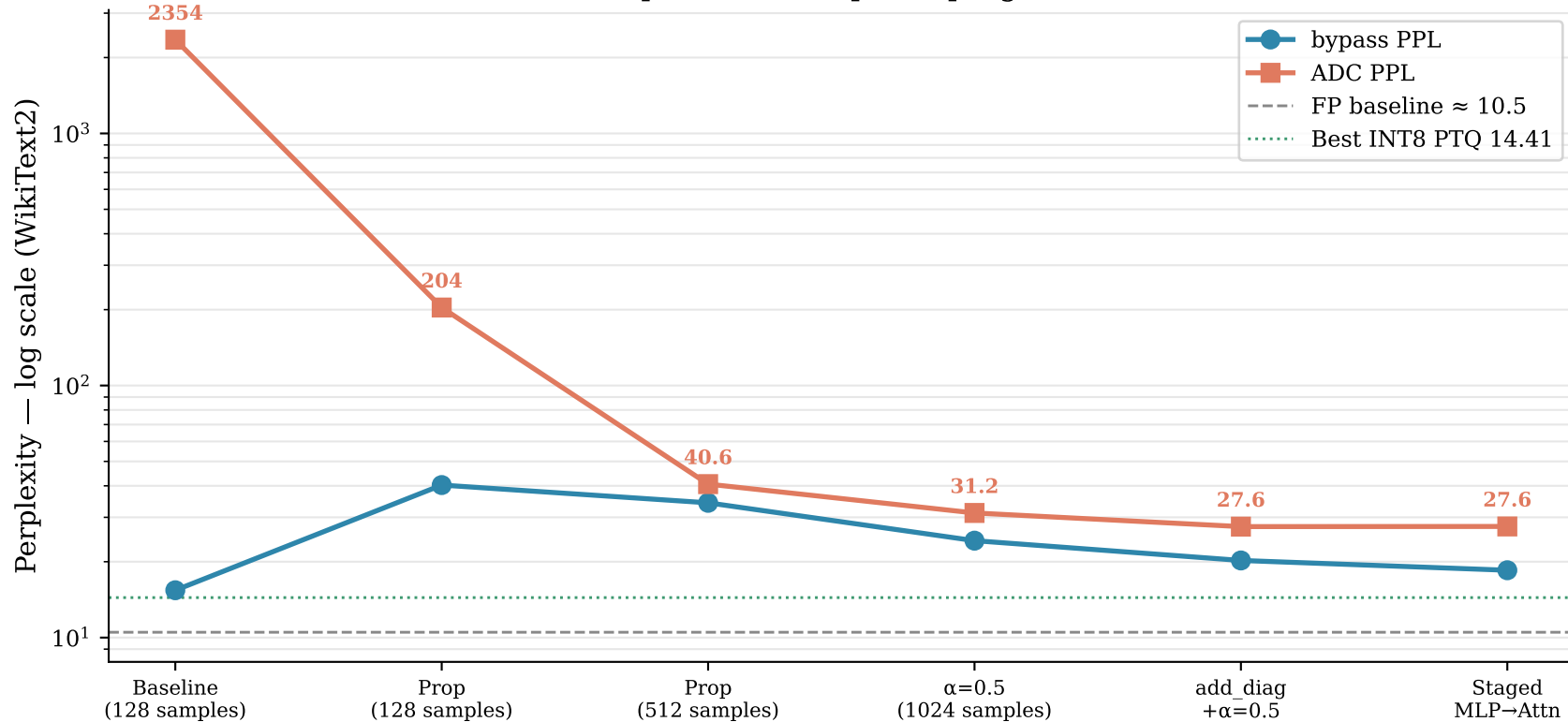
INT4 pure PTQ: stepwise progression
