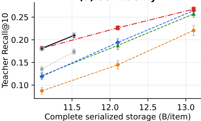
(a) Set fidelity
