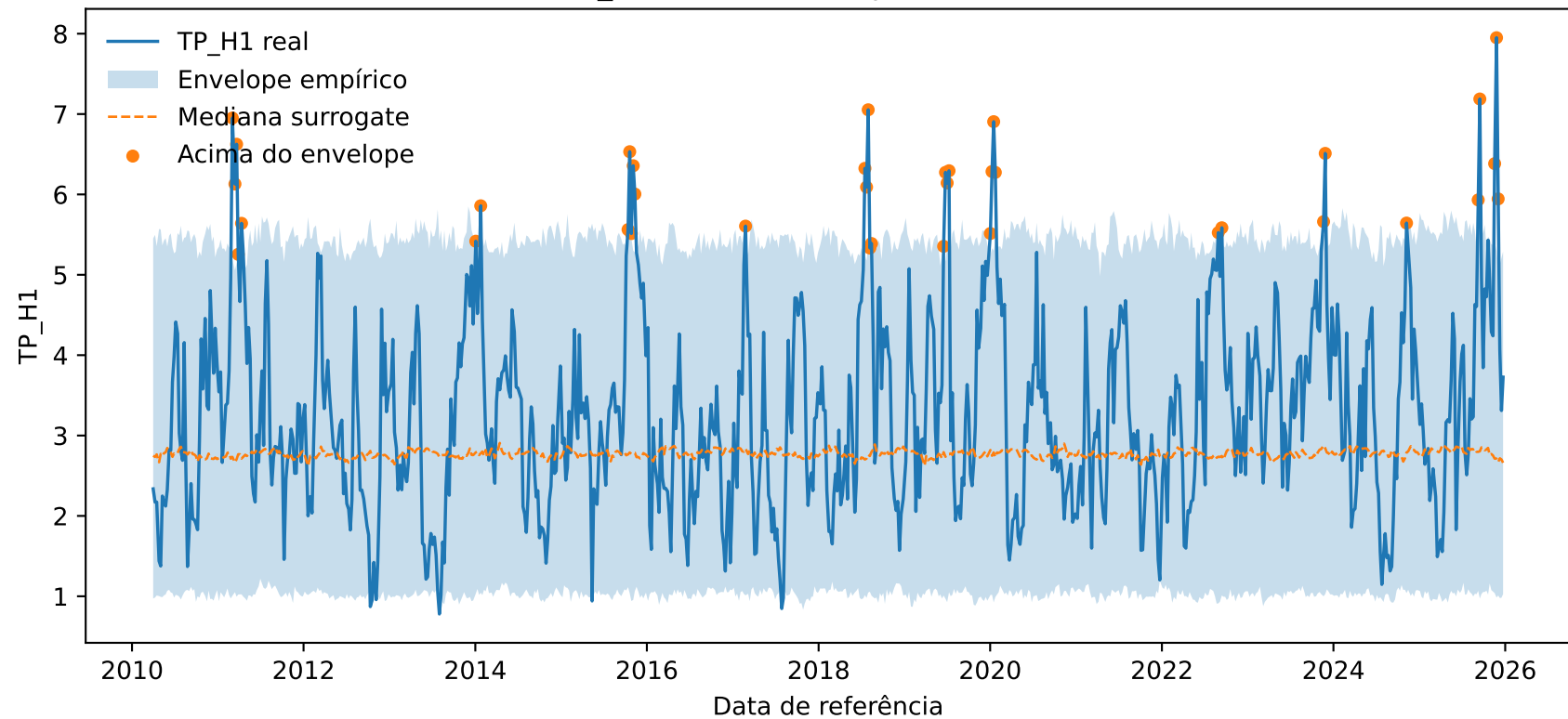
TP_H1 real vs envelope — ITUB4.SA
