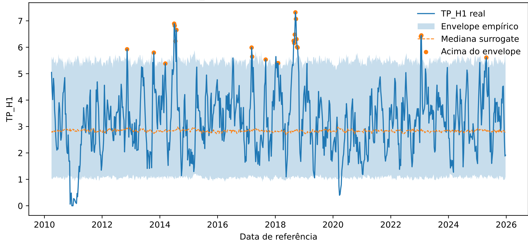
TP_H1 real vs envelope — LREN3.SA
