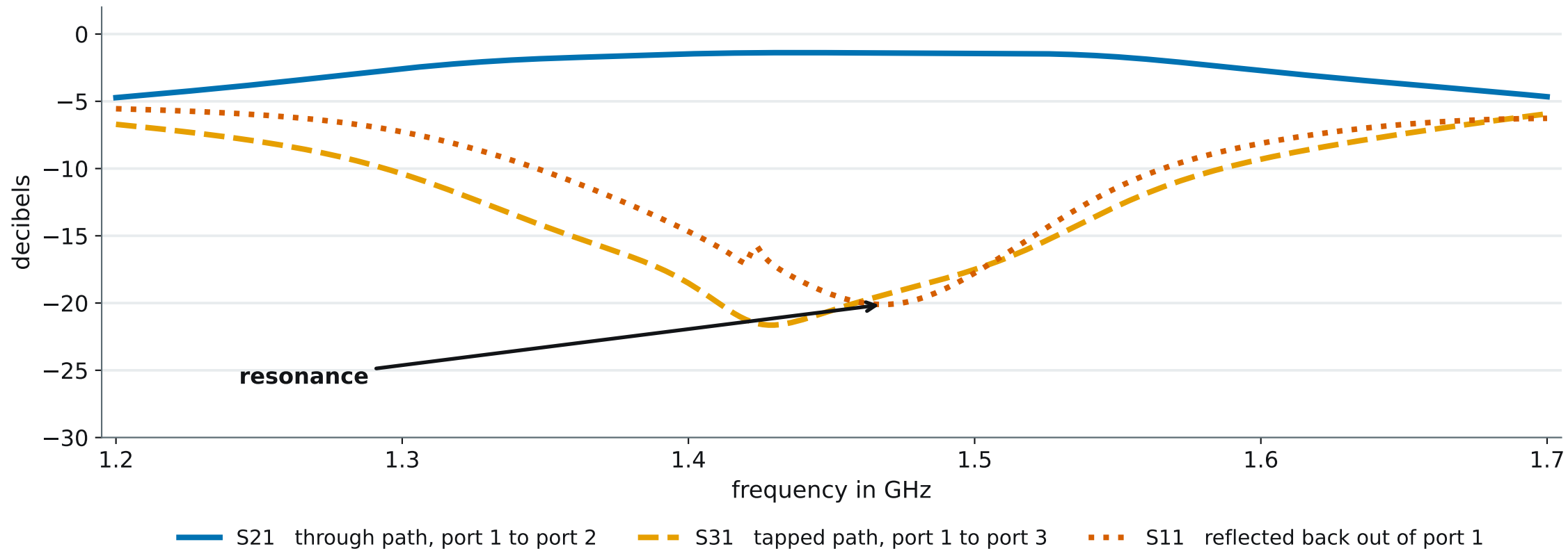
One board, measured at all 251 frequencies
