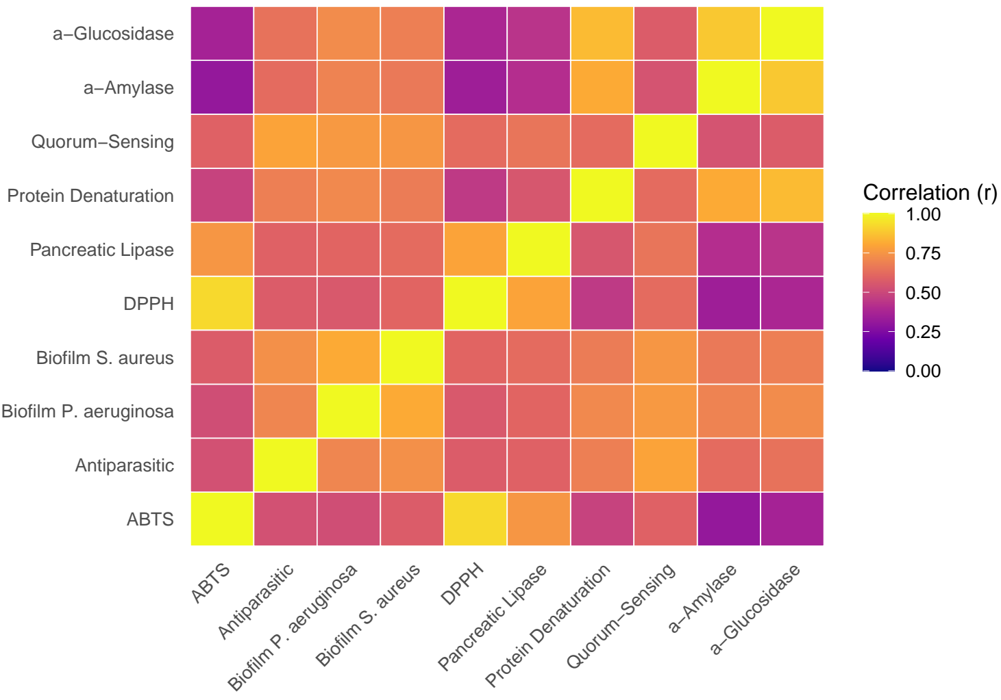
Correlation heatmap of biological activities
