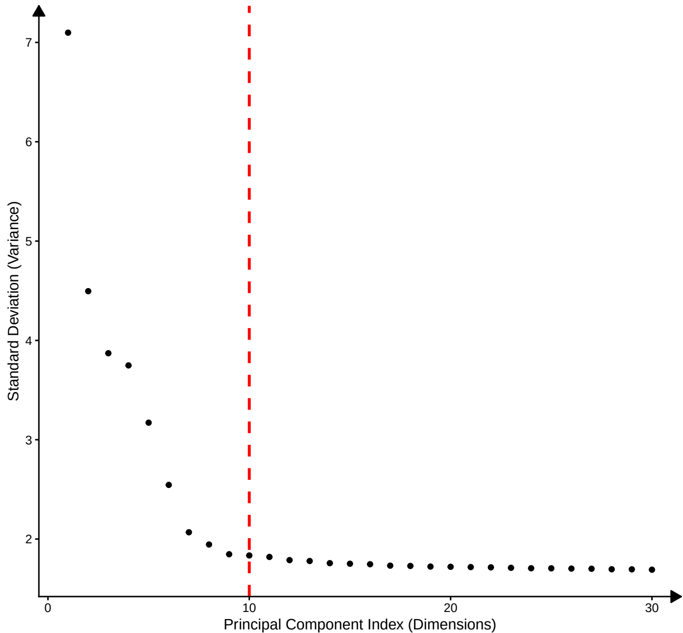
Figure 3: PCA Variance (Elbow Plot)
