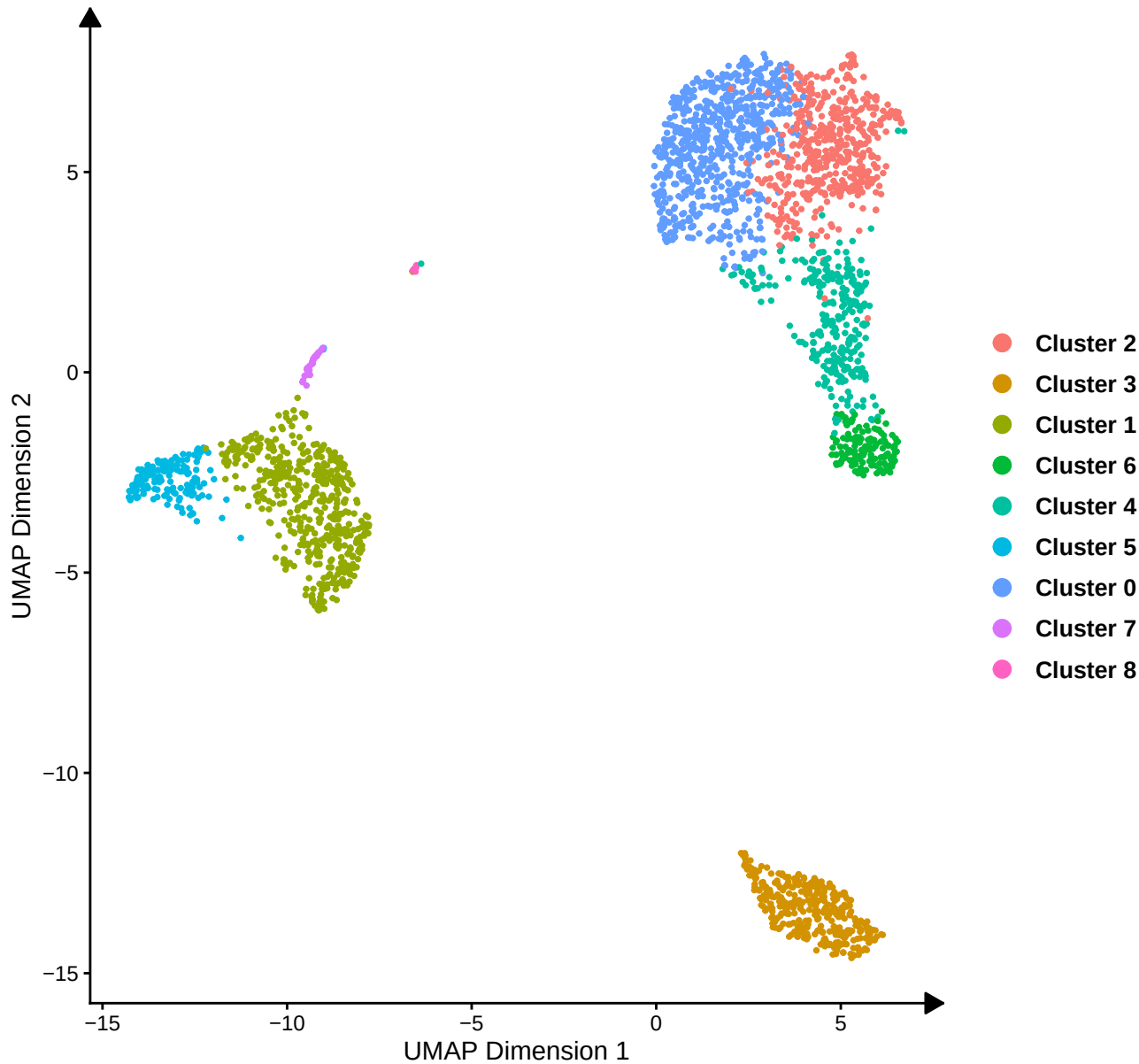
Figure 4: Mathematical Clustering
