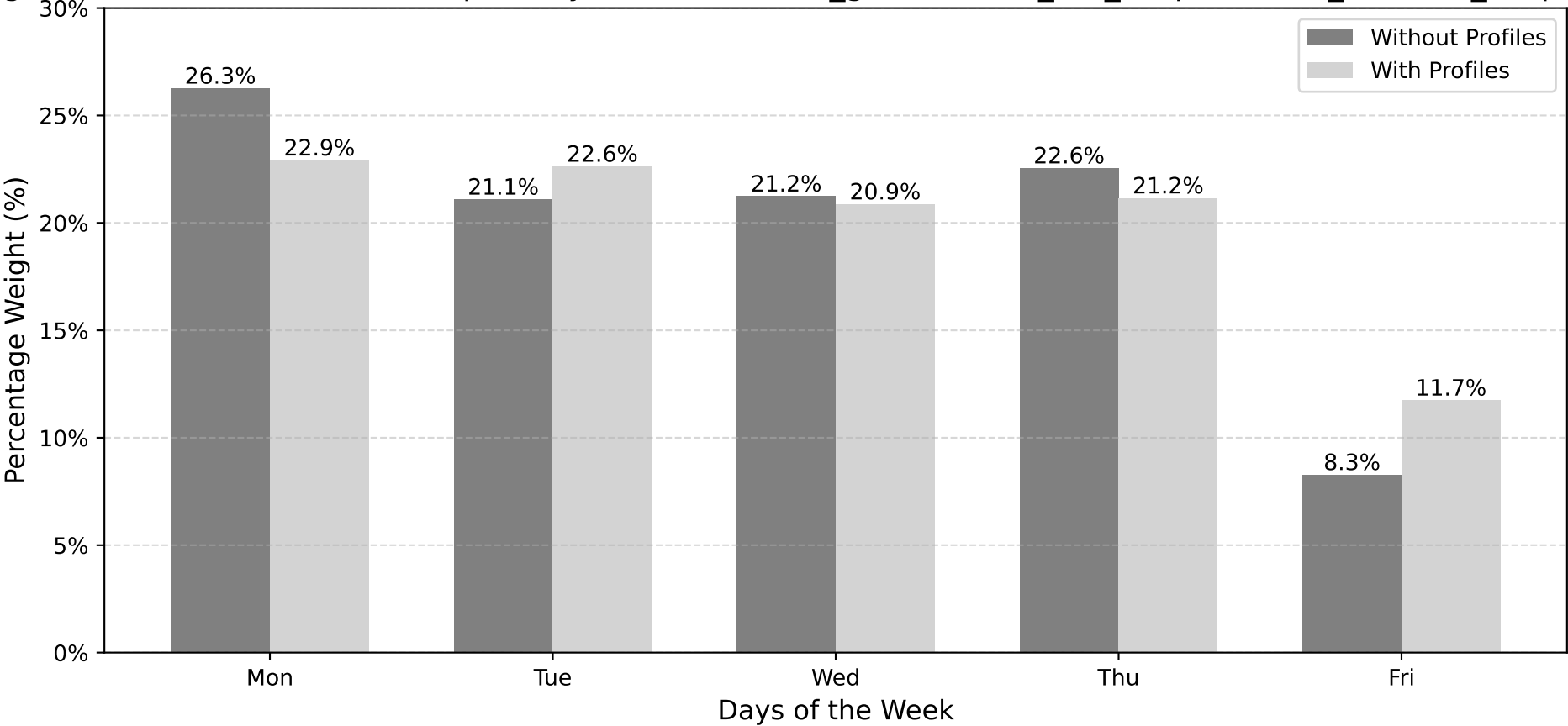
Percentage Weight with and without Profiles per Day (Full Data - var_gewicht1.33_var_frequenz1.33_mindest_frequenz2 - Non-Clustered)
