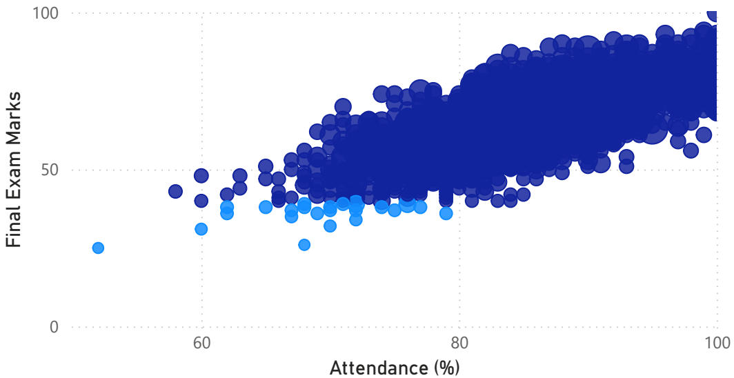
At-Risk Students (Low Attendance & Failed)
