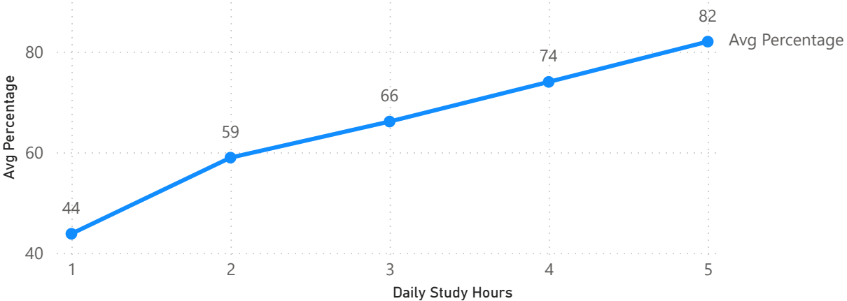
Study Hours vs Average Percentage
