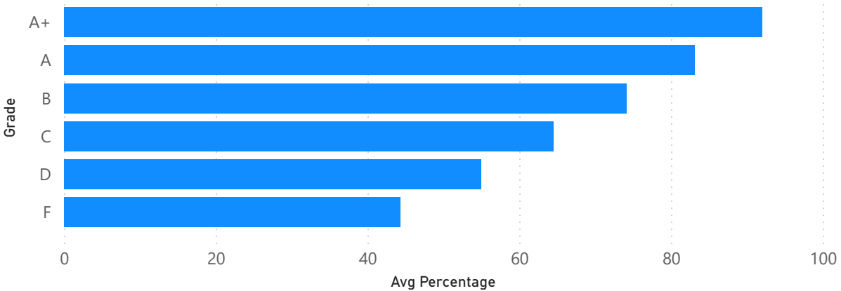
Internal Tests vs Final Exam Performance
