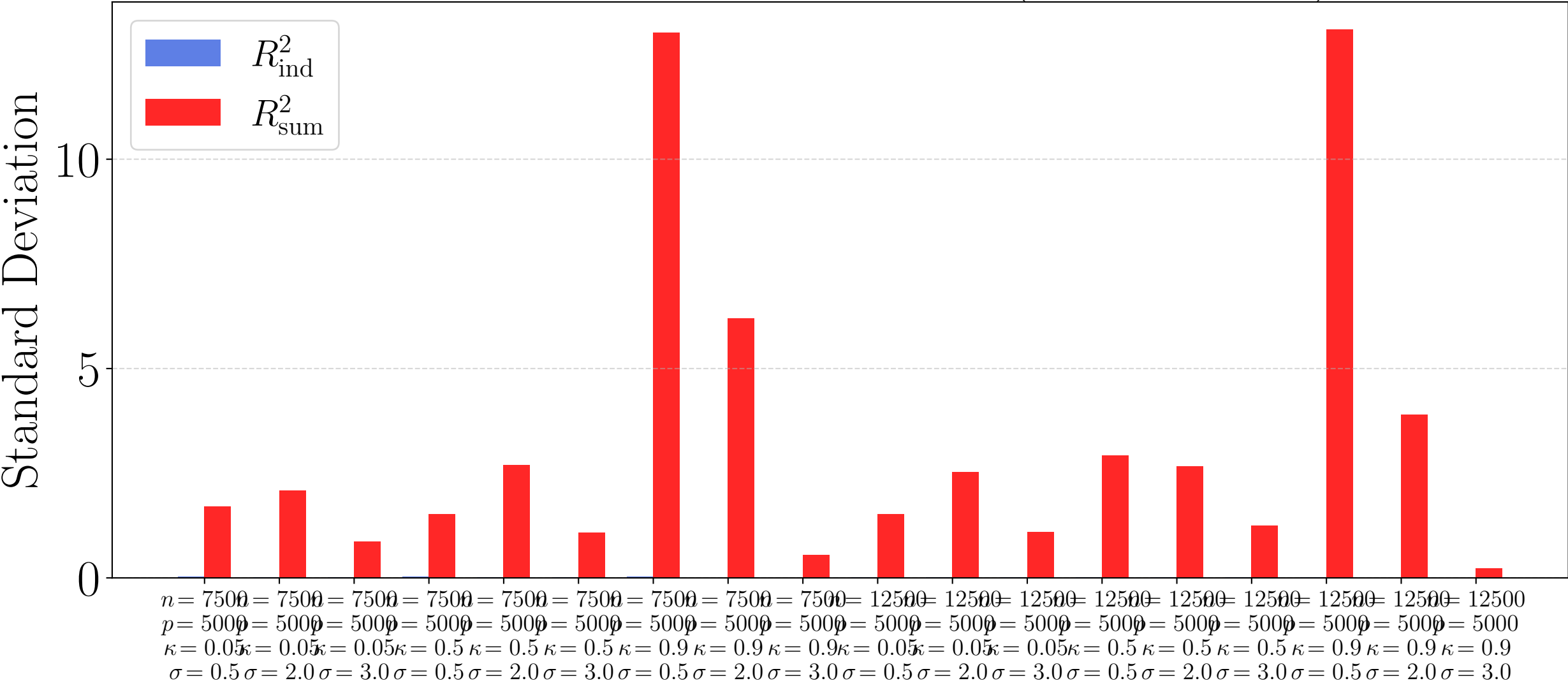
Std of R^2 across iterations ( n_w = 20000 )
